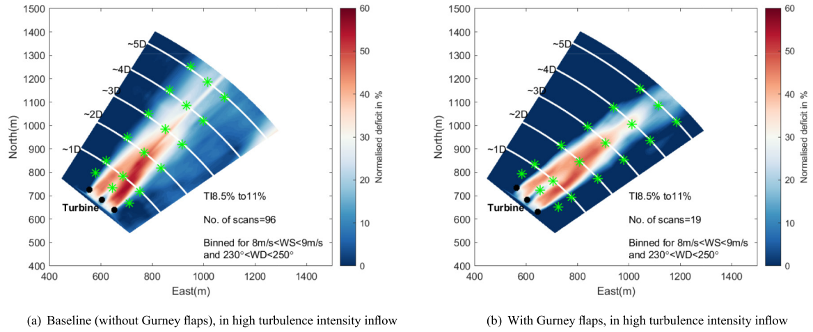
FIGURE 6 | Wake visualization at hub height for the 8 \text{ m/s} < U_{\infty,hub} < 9 \text{ m/s} wind speed bin. The green asterisks represent the assumed 1.5D wake width and the rotor hub line.
