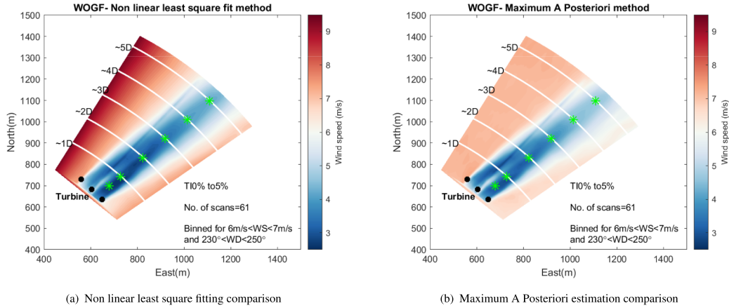
FIGURE B1 | Horizontal wind speed ( \sqrt{u^2 + v^2} ) example for a bin of ( 6\text{ m/s} < U_{\infty,hub} < 7\text{ m/s} ) (green asterisks: 50% span location).
