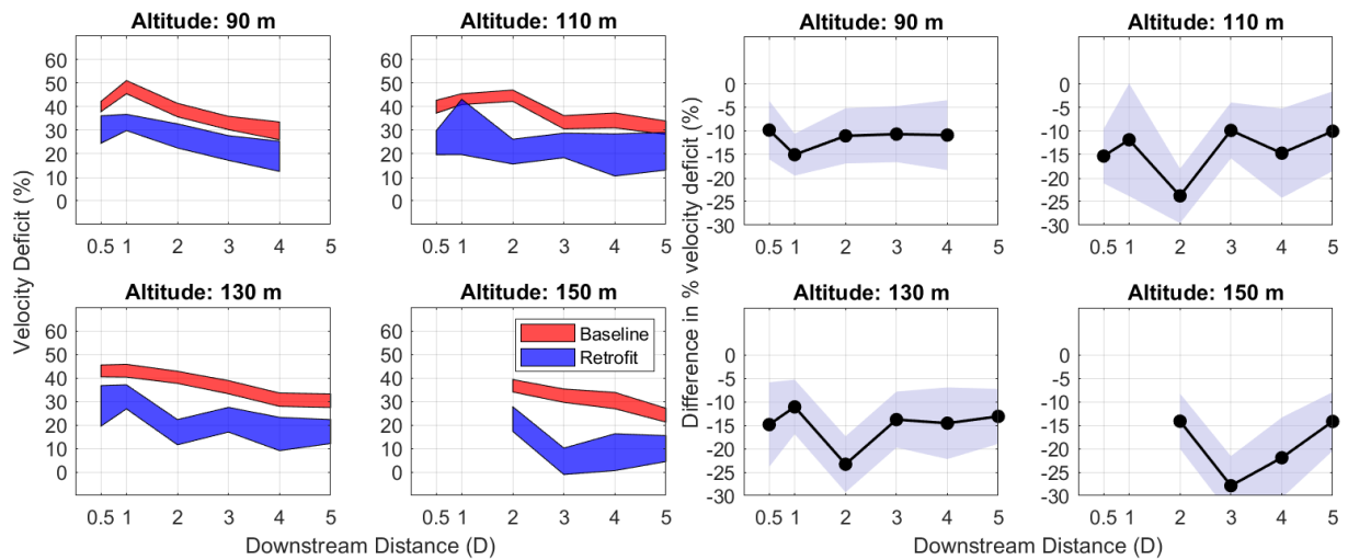
FIGURE 11 | Axial wake deficit profiles for the 10 \text{ m/s} < U_{\infty,hub} < 11 \text{ m/s} wind speed bin at different altitudes. The profiles are normalized with U_{\infty} at hub height. The patches indicate one time the standard error of the mean, on each side.
