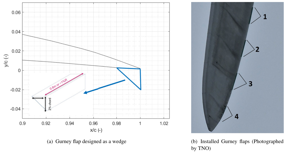
FIGURE 3 | Design and installation of the segmented Gurney flaps.
