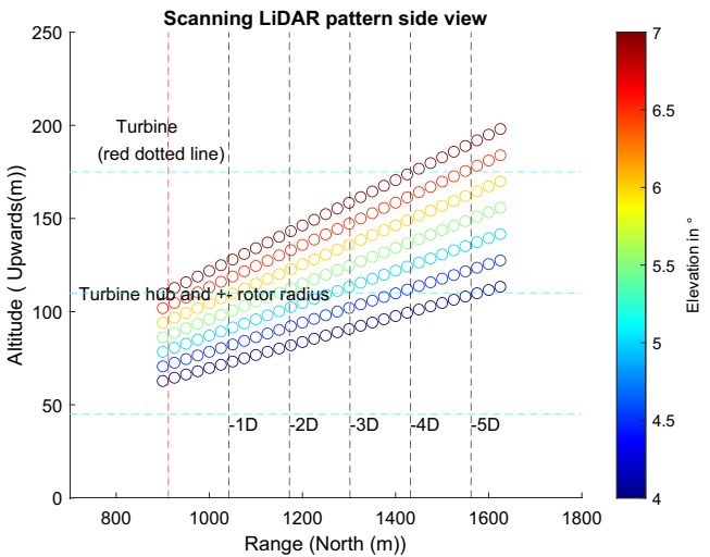
FIGURE A3 | Scanning LiDAR pattern side view.
