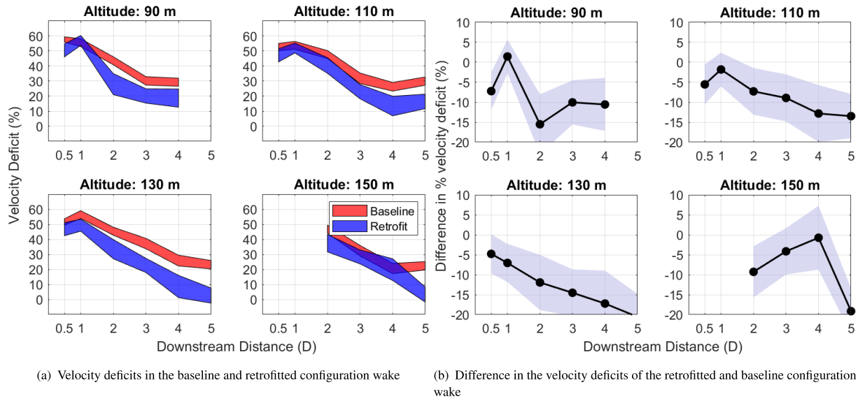
FIGURE 7 | Axial wake deficit profiles for the 8 \text{ m/s} < U_{\infty,hub} < 9 \text{ m/s} wind speed bin at different downstream distances. The profiles are normalized with U_{\infty} at hub height. The patches indicate one time the standard error of the mean, on each side.
