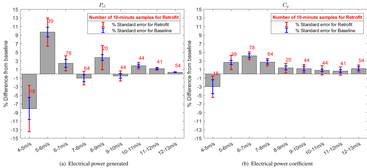
FIGURE 13 | Relative difference of power performance metrics, from baseline. The error bars denote the standard error as a percentage of the mean.
