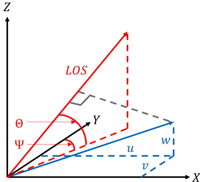
FIGURE A1 | Scanning LiDAR coordinate system.
