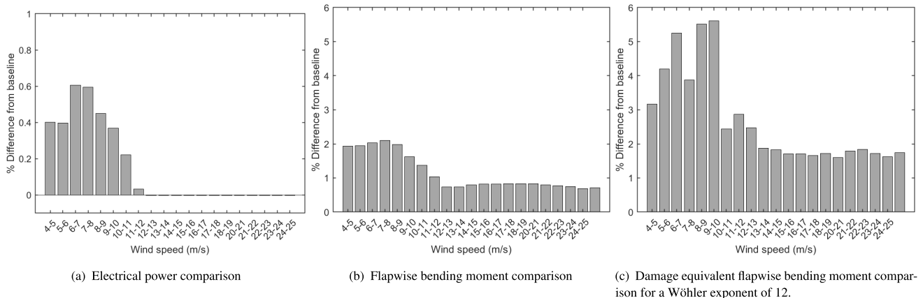
FIGURE 16 | Relative difference of turbine performance metrics, from baseline.
