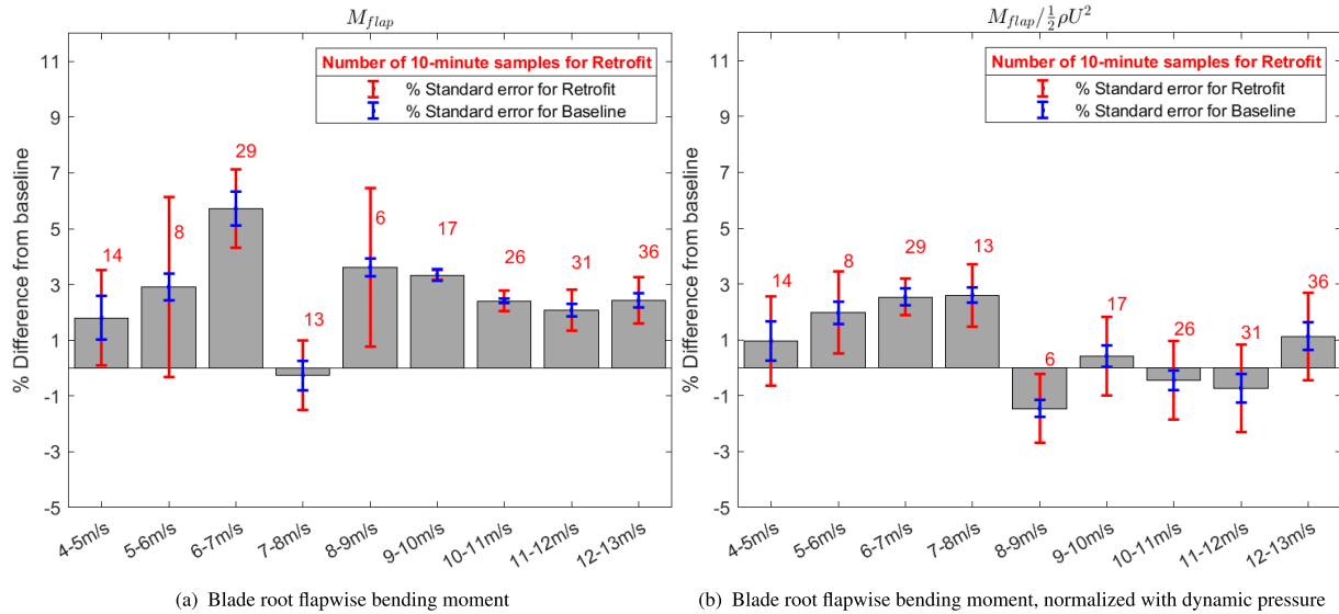
FIGURE 14 | Relative difference of loads, from baseline. The error bars denote the standard error as a percentage of the mean.
