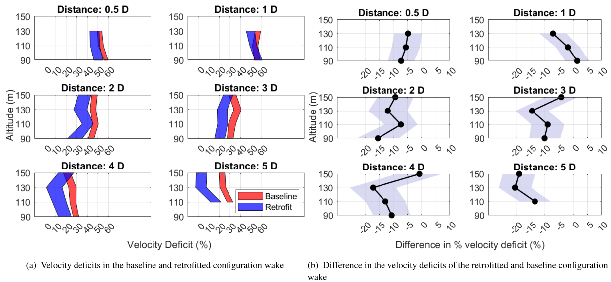
FIGURE 8 | Vertical wake deficit profiles for the 8 \text{ m/s} < U_{\infty, \text{hub}} < 9 \text{ m/s} wind speed bin at different downstream distances. The profiles are normalized with U_{\infty} at hub height. The patches indicate one time the standard error of the mean, on each side.
