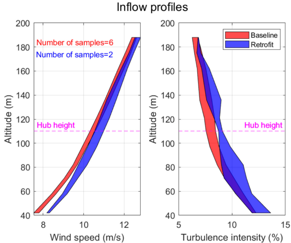
FIGURE 9 | Inflow profiles of wind speed and turbulence intensity for the 10 \text{ m/s} < U_{\infty, \text{hub}} < 11 \text{ m/s} wind speed bin. The patches indicate one time the standard error of the mean, on each side.
