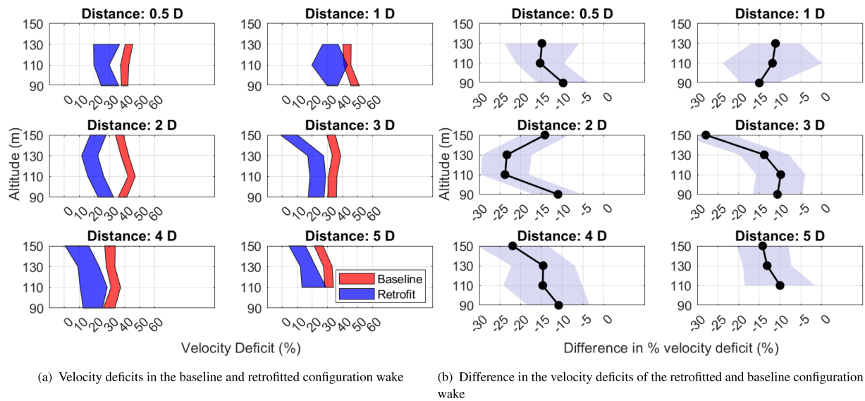
FIGURE 12 | Vertical wake deficit profiles for the 10 \text{ m/s} < U_{\infty,hub} < 11 \text{ m/s} wind speed bin at different downstream distances. The profiles are normalized with U_{\infty} at hub height. The patches indicate one time the standard error of the mean, on each side.
