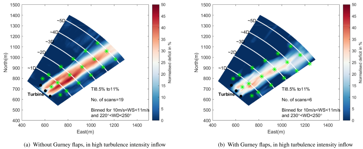
FIGURE 10 | Wake visualization at hub height for the 10 \text{ m/s} < U_{\infty,hub} < 11 \text{ m/s} wind speed bin. The green asterisks represent the assumed 1.5D wake width and rotor hub line.
