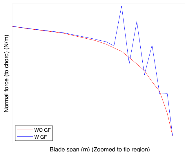
FIGURE 1 | Normal force distribution without and with segmented Gurney flaps on the 3.8-MW wind turbine blade (zoomed to the tip region).
