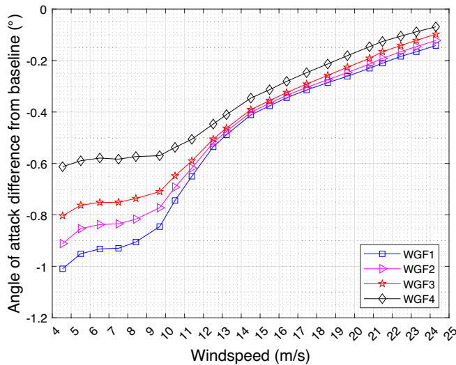
FIGURE 15 | Simulated difference in angle of attack from baseline at the different Gurney flap positions. WGF1-WGF4 represent the four different spanwise Gurney flap positions along the wind turbine blade tip as shown in Figure 3b.
