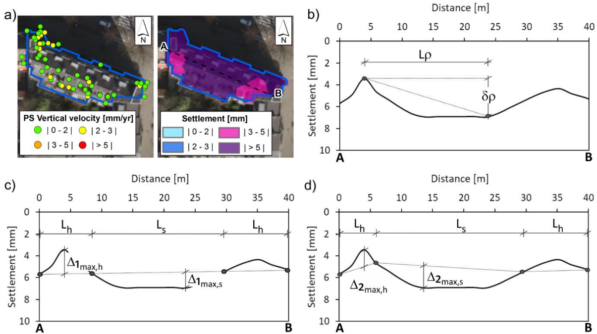
Fig. 3. Sketch synthesizing the computation of the DInSAR-derived SRI parameters: a) map of PS vertical velocity and cumulative settlement; b) differential settlement \delta\rho and L_p ; c) deflection ratio as \Delta_1/L_1 ; d) deflection ratio as \Delta_2/L_2 .
