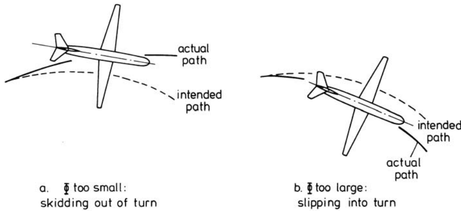
Figure 12.3 Turn with incorrect angle of bank
