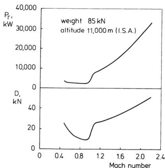
Figure 9.10 Power required and drag for supersonic airplane
