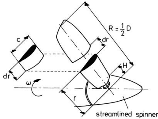
Figure 7.12 Blade element
