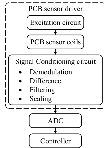
Fig. 4. Overall diagram of the designed sensor driver.
