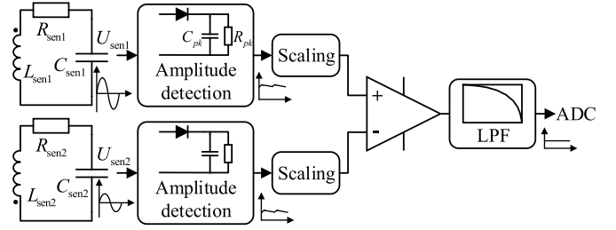
Fig. 7. Signal conditioning circuit.
