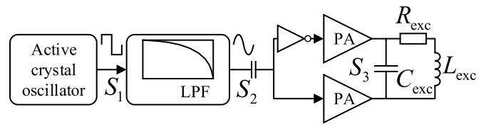
Fig. 5. Excitation circuit.
