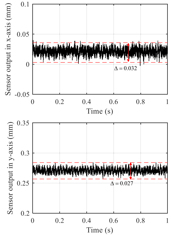
Fig. 11. Sensor outputs under rotor static suspension experiment.
