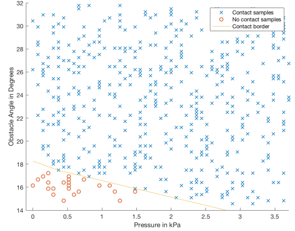
Fig. 11: The final sampling strategy that was applied to collect the training data. After introducing more contacted samples into the training set, the predictor can reconstruct very accurate shape of an obstructed actuator. the predictor gives a better reconstruction of obstructed actuator shapes, while maintaining its accuracy on unobstructed actuator shapes.
