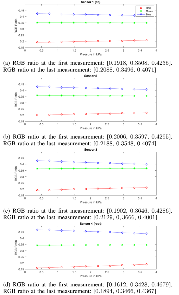
Fig. 7: RGB values of the four sensors plugged underneath the four bellows. The RGB ratio data is obtained by dividing the raw RGB values by the Clear value. For each sensor there is a clear increase in red and decrease in blue.
