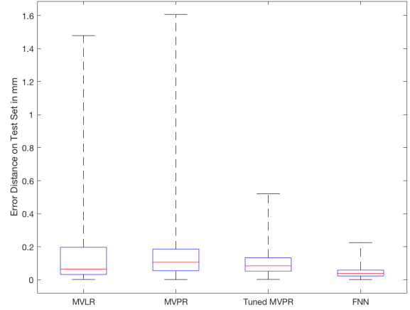
Fig. 16: The distances between the real positions and the positions predicted by the multivariate linear regression (MVLRL), the quadratic multivariate polynomial regression (MVPR), the tuned MVPR and the FNN. The predictions generated by the FNN have smaller errors.
