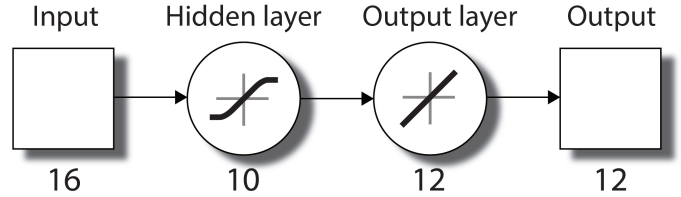
Fig. 12: Graphical representation of the Neural Network configuration used in our training process and the shape predictor.
