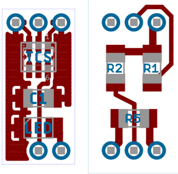
Fig. 17: The design of the upper PCB (left with dimension: 10.80 mm \times 5.08 mm) and the design of the lower PCB (right with dimension: 12.07 mm \times 6.35 mm).
