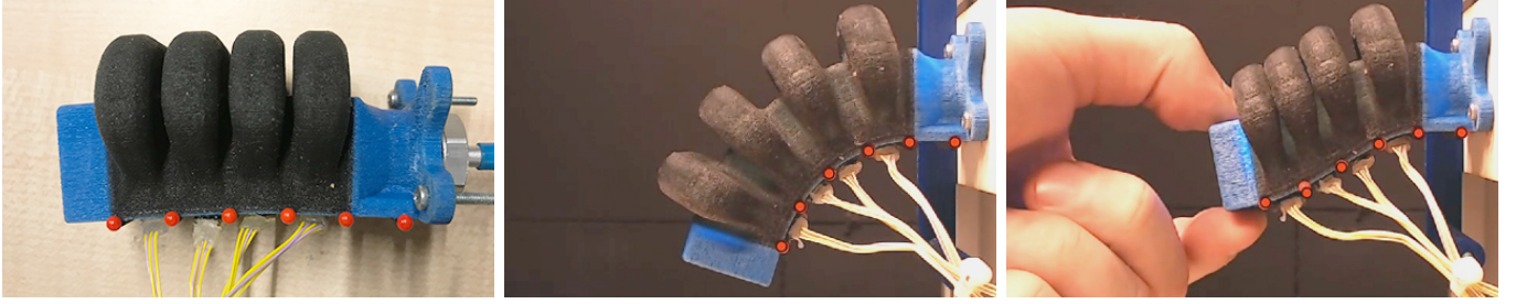
Fig. 1: A soft pneumatic actuator with red glass-headed pins inserted in the inextensible layer, serving as makers for the training of the neural network (left). The deformed shape is represented by the red dots, the locations of which are predicted from four color sensors embedded in the actuator (middle and right). Note that the predicted locations of the red dots accurately match the red pins, in the absence of object interaction (middle) and during interaction with objects (right).
