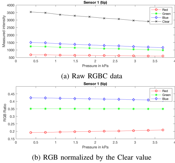
Fig. 6: (a) Raw RGBC data of a color sensor measured at pressure intervals during unobstructed bending. Besides a clear decrease in intensity due to an increased measuring distance, a change in color can be observed as well. (b) RGB normalized by the Clear value. The ratio of red gradually increases from 0.1918 to 0.2088, while the blue ratio decreases from 0.4235 to 0.4071.
