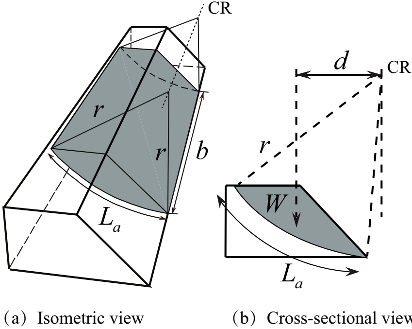
Figure 4.1: Diagrams showing the failure mass within a long 3D slope (based on Vanmarcke (1977b))
