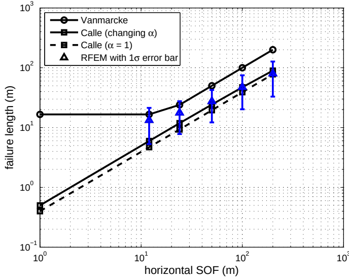
Figure 5.14: Potential failure length versus horizontal scale of fluctuation for the various models ( F_T = 1.30 , five RFEM results corresponding to \theta_h = 12, 24, 50, 100 and 200 m shown with their means and associated one \sigma error bars)
