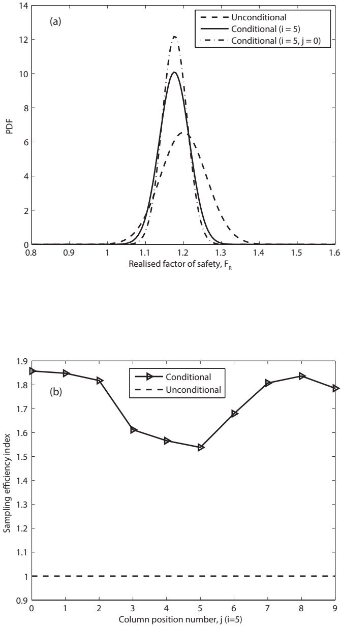
Figure 6.12: Influence of CPT location j during the second phase of site investigation (based on \theta_v = 1.0 m and 500 realisations per simulation): probability density function of realised factor of safety ( \xi = 6 ) (a); influence of CPT location j with i = 5 ( \xi = 6 ) (b)
