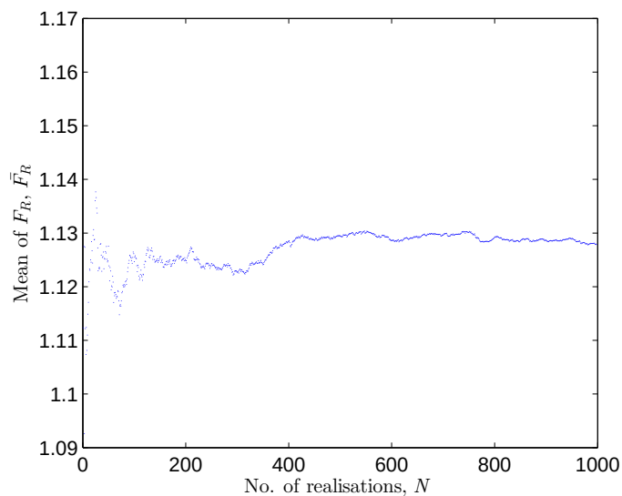
Figure B.13: Mean of the realised factor of safety versus number of MC realisations ( \theta_h = 100 m, L = 500 m)
