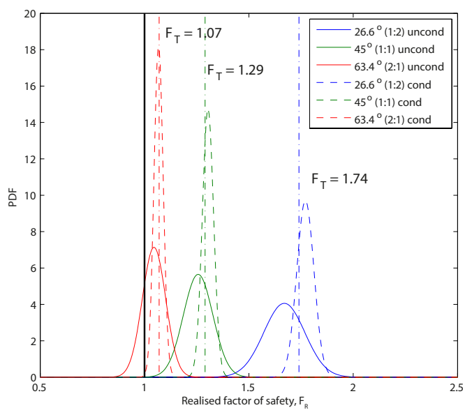
Figure 6.16: PDFs of realised factor of safety for three slopes, based on conditional and unconditional simulations (cond: conditional; uncond: unconditional)
