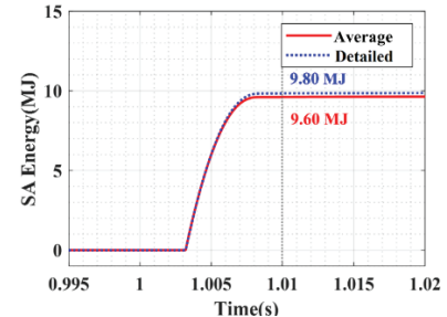
Fig. 5. Comparison of the energy absorbed in CB 1a during a terminal short circuit for both the average and the detailed VARC model
