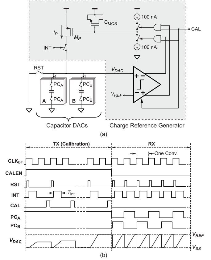
Fig. 7. (a) Schematic of the charge reference generator and (b) its timing diagram.
