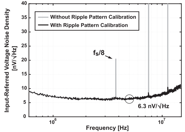
Fig. 16. Measured input-referred noise density spectrum of one subarray receiver.
