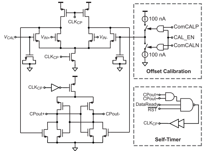
Fig. 10. Dynamic comparator with offset calibration.
