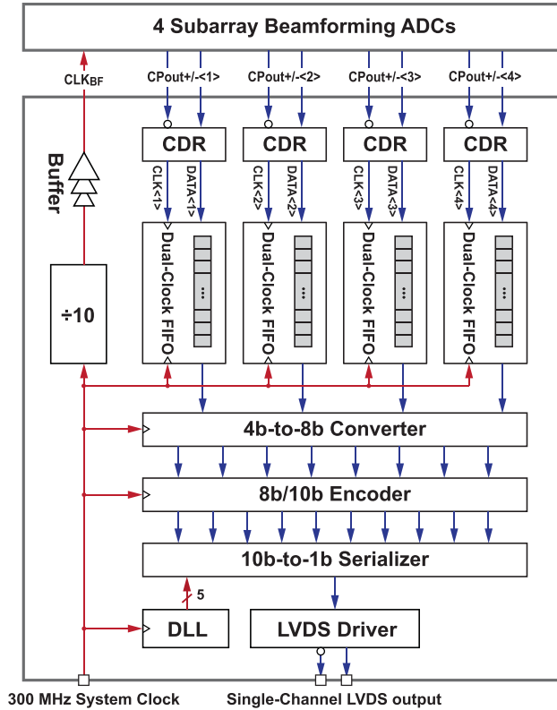
Fig. 5. Datalink architecture.
