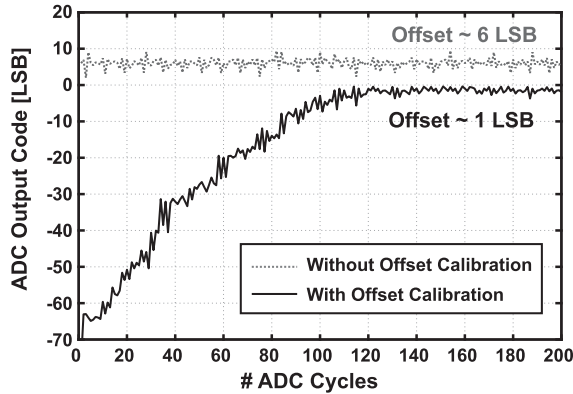
Fig. 18. Convergence of the background comparator offset calibration process.
