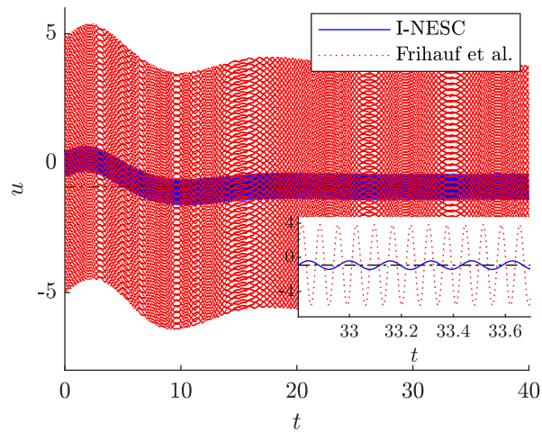
Figure 3.2: Input of the first agent under I-NESC (solid blue) and [7] (dotted red)
