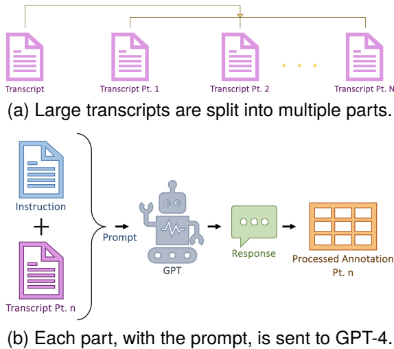
Figure 4: Generating annotation using GPT-4.
