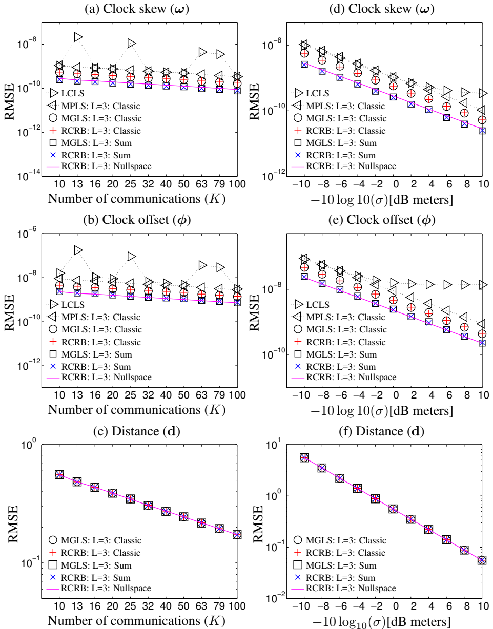
Figure 4.5: Mobile network: (Left) Varying K : RMSEs (and RCRBs) of (a) clock skew, (b) clock offset and (c) distance estimates, for varying number of communications ( K ) between the N = 5 mobile nodes for \sigma = 3.3\text{nS} (1 meter). (Right) Varying \sigma : RMSEs (and RCRBs) of (d) clock skew, (e) clock offset and (f) distance estimates for a cluster of mobile nodes, for varying noise ( \sigma ) on the time measurements with K = 10 number of communications.
