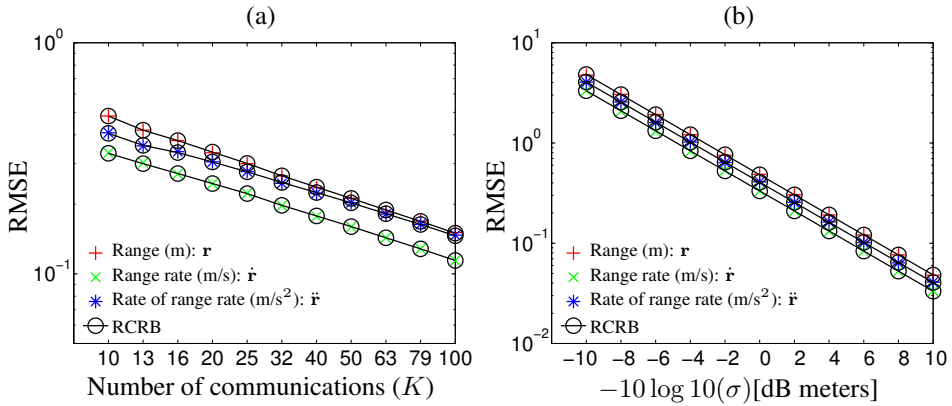
Figure 4.6: Mobile network: RMSEs of range parameters (a) for varying number of communications ( K ) between the nodes for \sigma = 1 meter and (b) for varying noise ( \sigma ) on the Time measurements with number of communication K = 10 .
