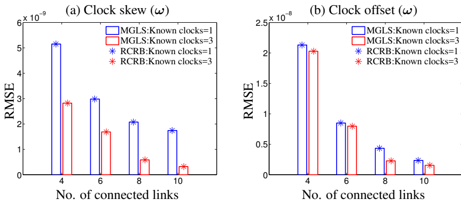
Figure 4.8: Effect of additional clocks on partially connected networks: RMSEs (and RCRBs) of (a) clock skew and (b) clock offset with K = 10 , L = 3 , \sigma = 3.3\text{nS} (1 meter), for a mobile network with varying number of connected links.
