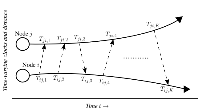
Figure 4.1: Asynchronous pair of mobile nodes : A generalized two-way ranging (TWR) scenario between a pair of asynchronous nodes in motion, where the nodes exchange K time stamps each. The curved lines symbolize the time-varying motion of the nodes, in addition to the independent clock drifts. See Remark 1.
