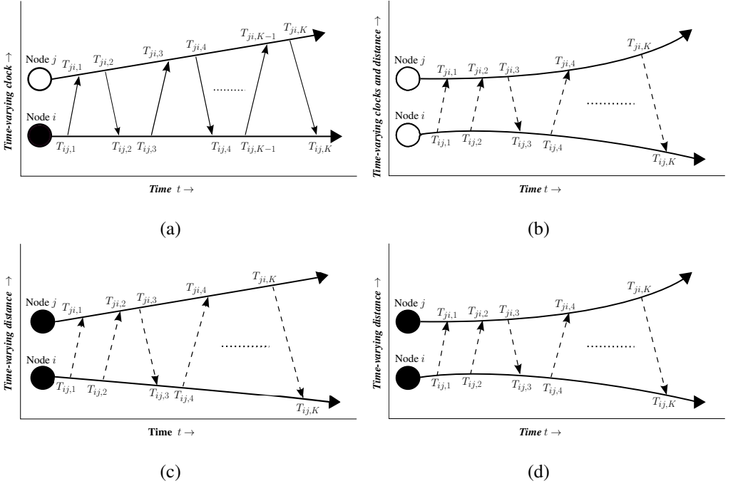
Figure 1.3: Generalization of two-way ranging to mobile nodes: (a) Classical two-way ranging between a pair of fixed asynchronous nodes, (b) Generalized two-way ranging (GTWR) between a pair of asynchronous mobile nodes (Chapter 4), (c) A pair of mobile nodes with linear independent velocities (Chapter 5), (d) A pair of mobile nodes with non-linear motion (Chapter 6). The shaded nodes indicate ideal clocks.
