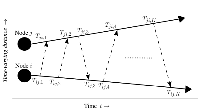
Figure 5.1: Illustration of a pair of mobile nodes in linear motion: A generalized Two-Way Ranging (TWR) between a pair of mobile nodes, where the solid-skewed lines indicate the linear motion of the nodes. During the linear motion, the nodes transmit and receive K time stamps, which are recorded at the respective nodes. Similar to [Rajan and van der Veen 2011; Rajan and van der Veen 2013; Rajan and van der Veen 2015], we levy no constraints on the sequence, direction or number of communications.
