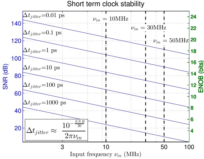
Figure 3.2: Short-term clock stability: Limiting cases of the SNR and corresponding ENOB due to jitter t_{\text{jitter}} versus input frequency \nu_{in} . The demarcation lines at 10MHz, 30MHz and 50MHz show the maximum input frequencies of the DARIS, OLFAR and FIRST systems at \nu_{in} = 30\text{MHz} .
