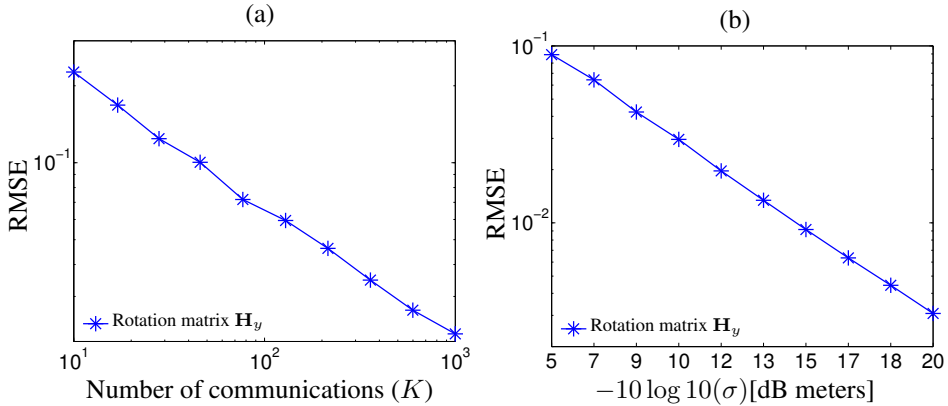
Figure 5.4: RMSEs of rotation matrix (a) for varying number of communications ( K ) between the nodes for \sigma = 1 meters and (b) for varying noise ( \sigma ) on the time measurements with number of communication K = 10 .
