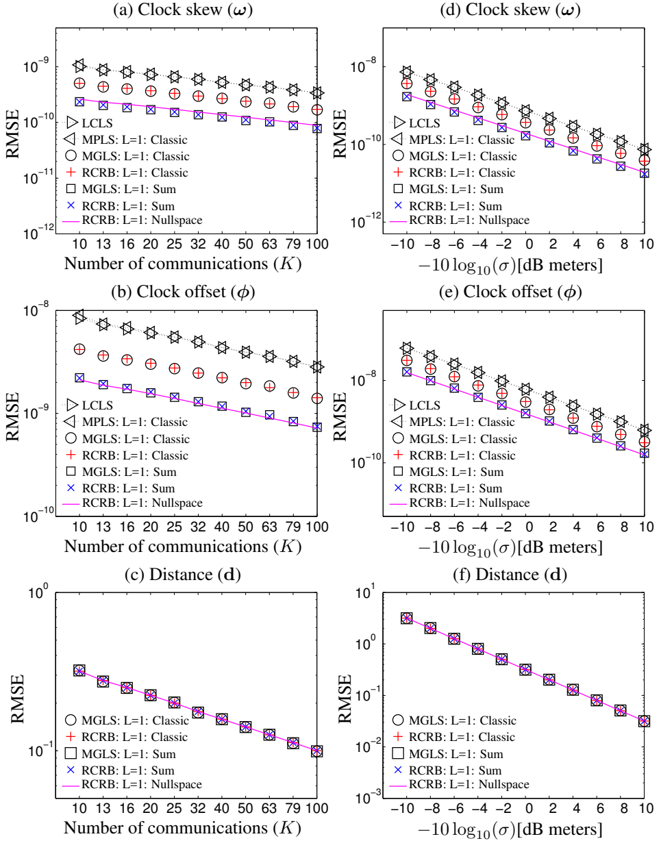
Figure 4.4: Immobile network: (Left) Varying K : RMSEs (and RCRBs) of (a) clock skew, (b) clock offset and (c) distances for varying number of communications ( K ) between the N = 5 fixed nodes for \sigma = 3.3nS (1 meter). (Right) Varying \sigma : RMSEs (and RCRBs) of (d) clock skew, (e) clock offset and (f) distances for a cluster of fixed nodes, for varying noise ( \sigma ) on the time measurements with K = 10 number of communications.
