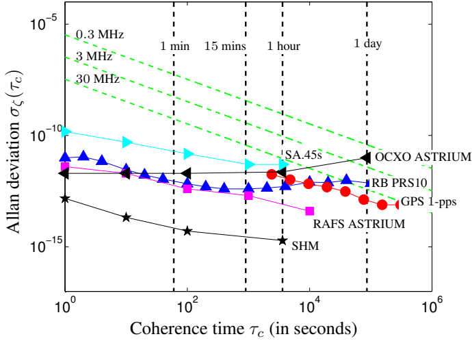
Figure 3.1: Long-term clock stability: Allan deviations of free running clocks are plotted versus the coherence time (in green) for various input frequencies \nu_i . The map is overlaid with Allan deviations of potential clocks for potential space-based low frequency arrays namely PRS-10 Rubidium [Stanford 2006], RAFA ASTRUM [Droz et al. 2007], GPS 1pps [Lombardi et al. 2001], OXCO ASTRUM [Airbus Defense and Space 2012], SA.45s CSAC and Space Hydrogen Maser (SHM) [Goujon et al. 2010].
