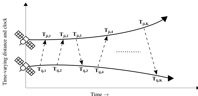
Figure 2.6: Dynamic ranging : A generalized two-way ranging (GTWR) scenario between a pair of asynchronous mobile satellite nodes where the nodes transmit and receive asymmetrically [Rajan and van der Veen 2015]. See Chapter 4.
