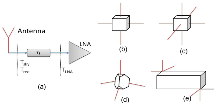
Figure 2.2: Space-based antenna model and potential configurations : (a) System model of the observation Antenna connected to an LNA (b) Configuration of a dipole antenna on a cubesat (c) Configuration of a tripole antenna in a cubesat (d) Configuration of an antenna with four monopoles (e) A dipole antenna placed on the opposite ends of a 3-cubesat.
