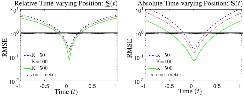
Figure 6.6: Error on position over time: RMSEs of (left) relative position \underline{\mathbf{S}}(t) and (right) absolute position \mathbf{S}(t) over time for K = [50, 100, 500] communications between a cluster of N = 10 mobile nodes, with \sigma = 1 meter.
