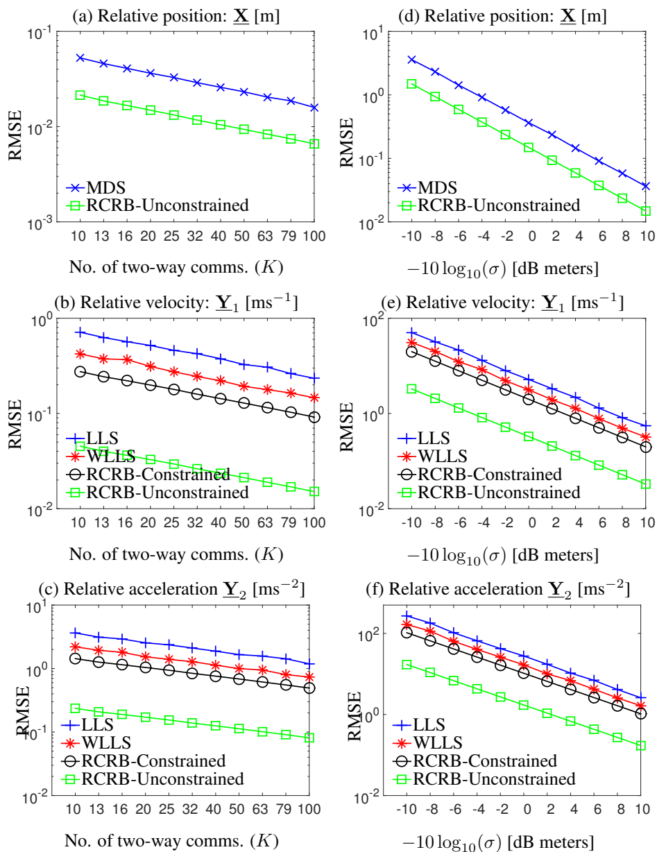
Figure 6.3: Relative Kinematics: Varying K : RMSEs (and RCRBs) of (a) Relative position ( \underline{\mathbf{X}} ), (b) Relative velocity ( \underline{\mathbf{Y}}_1 ) and (c) Relative acceleration ( \underline{\mathbf{Y}}_2 ) for varying number of communications ( K ) for \sigma = 0.1 meters. Varying \sigma : RMSEs (and RCRBs) of (d) Relative position ( \underline{\mathbf{X}} ), (e) Relative velocity ( \underline{\mathbf{Y}}_1 ) and (f) Relative acceleration ( \underline{\mathbf{Y}}_2 ) for K = 10 , and where the noise on the time markers ( \sigma ) is varied.
