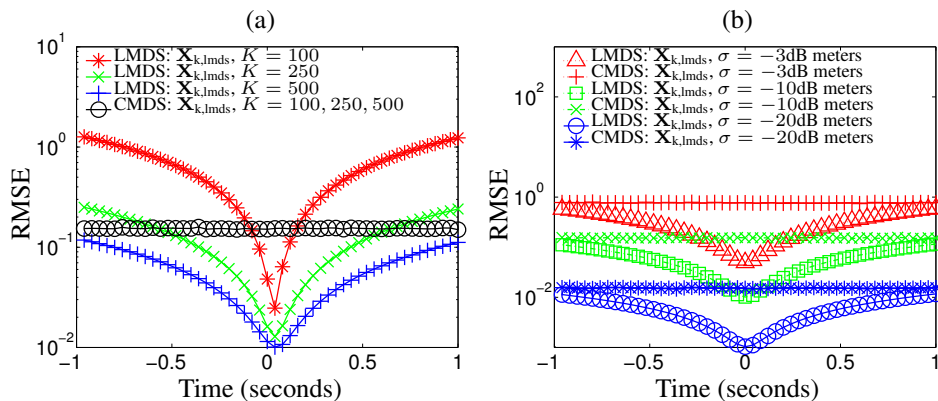
Figure 5.5: RMSE of relative positions over time t_k around t_0 = 0 (a) for K = [100, 250, 500] communication links with noise on time measurements \sigma = 1 meters and (b) for varying signal-to-noise ratio \sigma = [-3, -10, -20] dB meter with fixed K = 500 .
