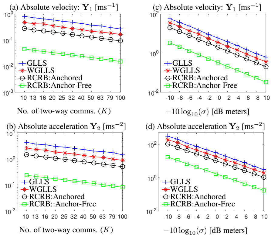
Figure 6.5: Absolute kinematics: Varying K : RMSEs (and RCRBs) of (a) Absolute velocity ( \mathbf{Y}_1 ) and (b) Absolute acceleration ( \mathbf{Y}_2 ) for varying number of communications ( K ) between the N = 10 mobile nodes for \sigma = 0.1 meters. Varying \sigma : RMSEs (and RCRBs) of (c) Absolute velocity ( \mathbf{Y}_1 ) and (d) Absolute acceleration ( \mathbf{Y}_2 ), for a network of N = 10 exchanging K = 10 timestamps, where the Noise on the time markers ( \sigma ) is varied.
