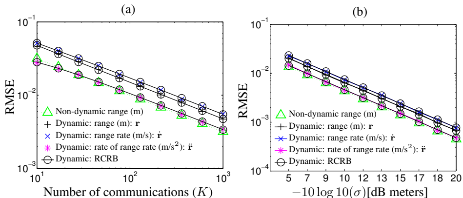
Figure 5.2: RMSEs of range parameters (a) for varying number of communications ( K ) between the nodes for \sigma = 1 meter and (b) for varying noise ( \sigma ) on the time measurements with number of communication K = 10 .
