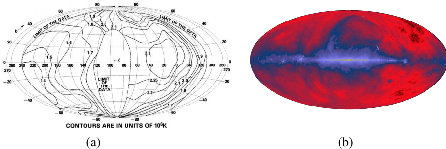
Figure 1.2: Status of ultra-long wavelength radio astronomy : The all sky map as observed by (a) Lunar orbiter radio astronomy explorer 2 (RAE-2) at 4.7 MHz [Novaco and Brown 1978] and by (b) Jordell Bank + Parks + Effelsberg at 408MHz [Haslam et al. 1982].
