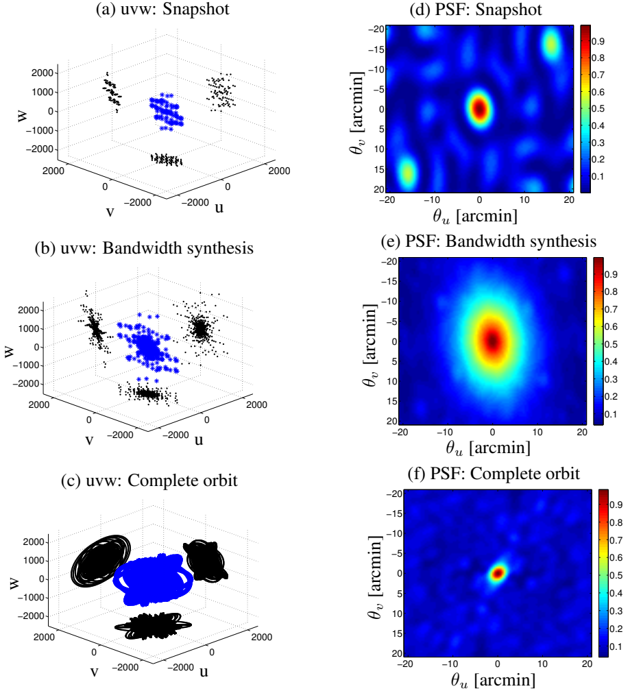
Figure 2.1: Baseline and PSF simulations: The aperture filling of a 9-satellite ULW array for an Earth leading orbit around the Sun (a)-(c), to illustrate the effect of the sampling space on the normalized Point Spread Function (PSF) (d)-(f). The uvw coverage for the 3-D array of satellites at \nu = 10\text{MHz} (a) for a single snapshot N_t = 1 along with (d) the corresponding PSF. Bandwidth synthesis is illustrated in (b) which shows the uvw coverage of single snapshot using 10 frequency bins uniformly distributed in the range 1 - 10 MHz with (e) the resultant PSF. The subfigures (c) and (f) show the uvw and the corresponding PSF, for an entire orbit around the sun at 10MHz with a single observation each day, i.e., 365 snapshots.
