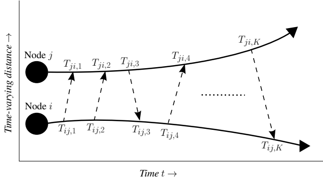
Figure 6.1: Illustration of a pair of mobile nodes in non-linear motion : A generalized two-way ranging (TWR) scenario between a pair of mobile nodes, where the nodes exchange K time stamps asymmetrically with each other. The curved lines symbolize the non-linear motion of the mobile nodes with time. Unlike our previous model in Chapter 5, which considered only linear independent velocities of the nodes, in this chapter we consider non-linear motion of the nodes.
