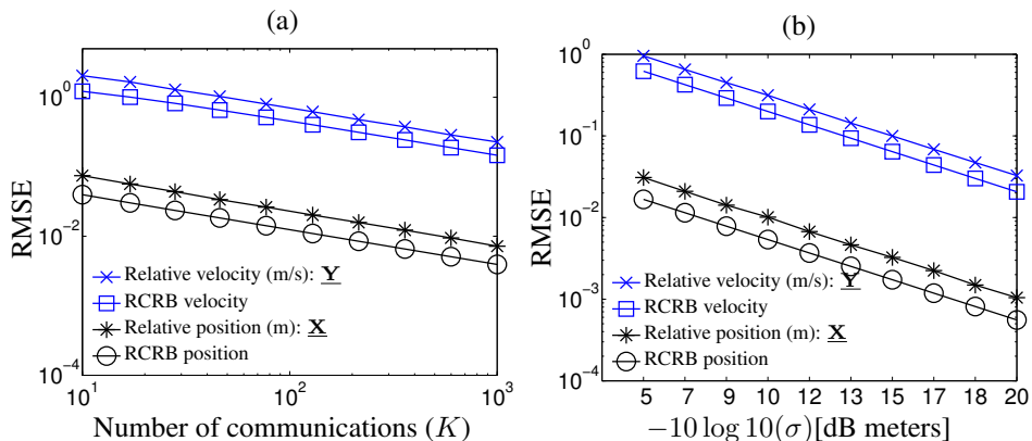
Figure 5.3: RMSEs of relative positions and velocities (a) for varying number of communications ( K ) between the nodes for \sigma = 1 meter and (b) for varying noise ( \sigma ) on the time measurements with number of communication K = 10 .
