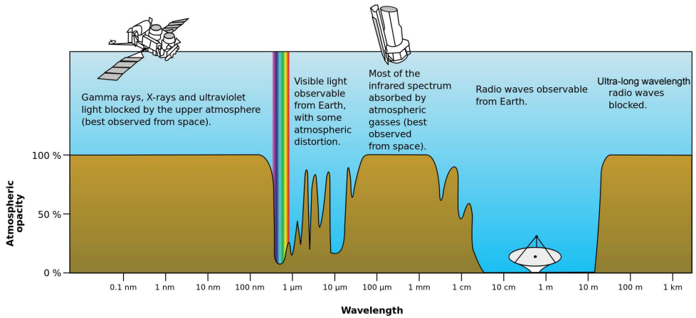
Figure 1.1: Atmospheric opacity : The opacity (or transparency) of the Earth's atmosphere at various wavelengths across the electromagnetic spectrum [Wikipedia 2008].
