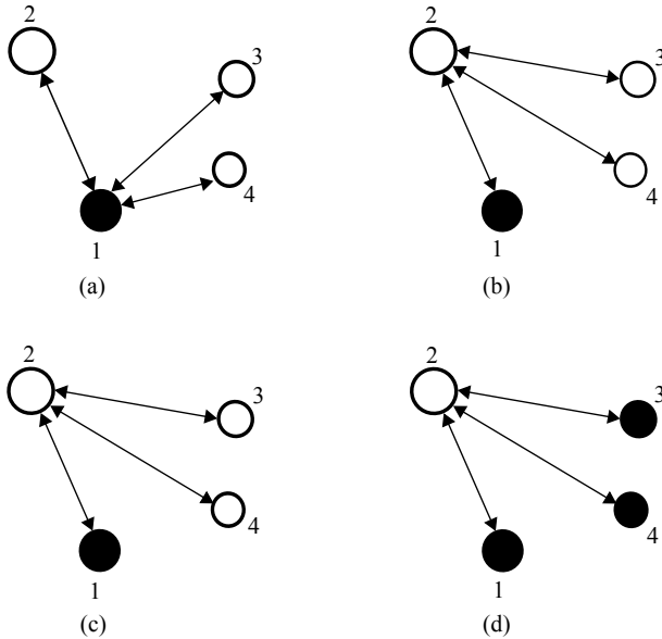
Figure 4.3: Illustration of feasible networks for the proposed algorithms : Four networks with N = 4 nodes each capable of two-way communication. The nodes shaded in black are the clock references. The 4 networks are illustrative examples where MGLS algorithm (and thus the constrained formulation) can be applied for network wide clock synchronization, despite missing communication links and multiple clock references.
