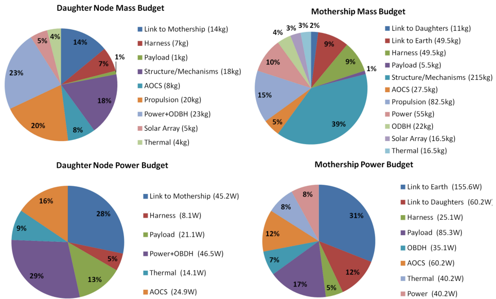
Figure 2.7: Mass and power budget analysis of the DARIS mission: The DARIS mission consists of 8 Daughter nodes and 1 centralized mothership. The mass (and power) of each Daughter satellite and Mothership was estimated to be 100kg (160W) and 550kg (502W) respectively [Boonstra et al. 2011].
