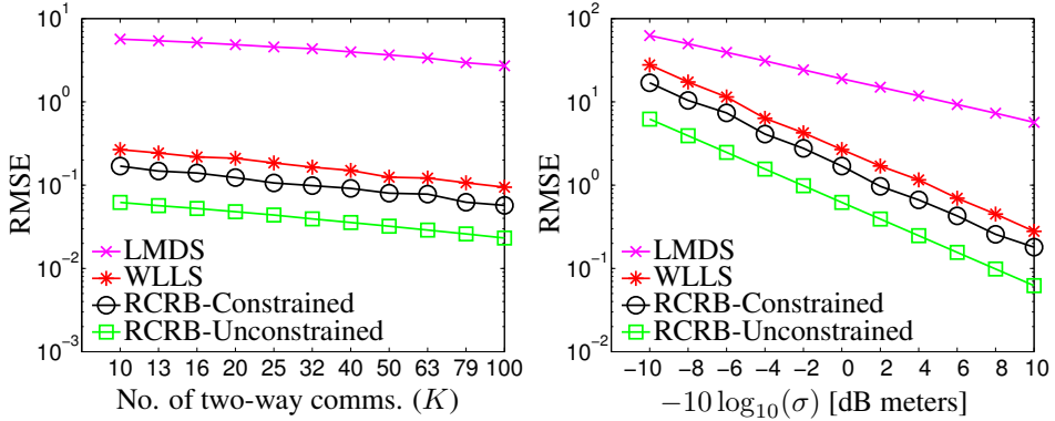
Figure 6.4: Comparison of relative velocity estimators : RMSEs (and RCRBs) of relative range parameters \mathbf{Y}_1 for (left) varying number of communications ( K ) for \sigma = 0.1 meters and (right) varying \sigma between the N = 10 mobile nodes.
