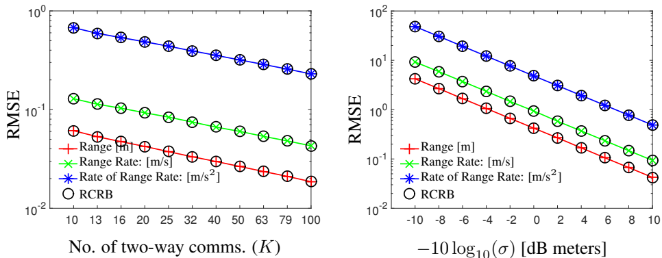
Figure 6.2: Range parameters: (Left) Varying K : RMSEs (and RCRBs) of relative range parameters ( \mathbf{r} , \dot{\mathbf{r}} , \ddot{\mathbf{r}} ) for varying number of communications ( K ) between the N = 10 mobile nodes for \sigma = 0.1 meters. (Right) Varying \sigma : RMSEs (and RCRBs) of relative range parameters ( \mathbf{r} , \dot{\mathbf{r}} , \ddot{\mathbf{r}} ) for a network of N = 10 exchanging K = 10 timestamps, where the noise on the time markers ( \sigma ) is varied. Unlike our previous experiments [Rajan, Leus and van der Veen 2015; Rajan and van der Veen 2015] (See Chapter 4 and Chapter 5), we consider acceleration in the current setup.
