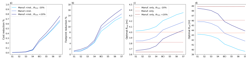
Figure 4. Sensitivity analysis on wall thickness. a) cost reduction and b) footprint reduction with respect to designs obtained minimising only fabrication costs. c) optimal R_{out} and d) optimal R_{off} obtained for all the cases reported in Table 4, considering both manufacturing and installation costs (solid lines), and for the manufacturing-only case (dashed lines)
