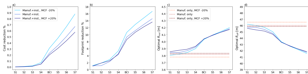
Figure 5. Sensitivity analysis on MCF . a) cost reduction and b) footprint reduction with respect to designs obtained minimising only fabrication costs. c) optimal R_{out} and d) optimal R_{off} obtained for all the cases reported in Table 4 considering both manufacturing and installation costs (solid lines), and for the manufacturing-only case (dashed lines)
