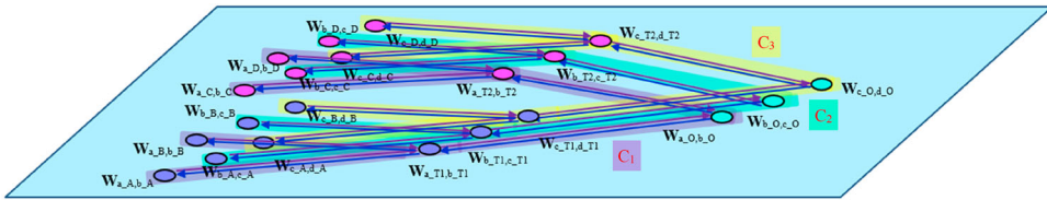
Figure 7. Full integration of feed forward learning and feedback learning. Three strongly connected components C_1 for all connections a \rightarrow b (purple highlighted), C_2 for all connections b \rightarrow c (green highlighted), C_3 for all connections c \rightarrow d (yellow highlighted). These three components have no mutual connections and therefore have mutually independent but internally common equilibrium values.
