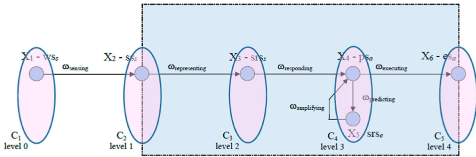
Figure 3. Stratified strongly connected components for the example network model.
