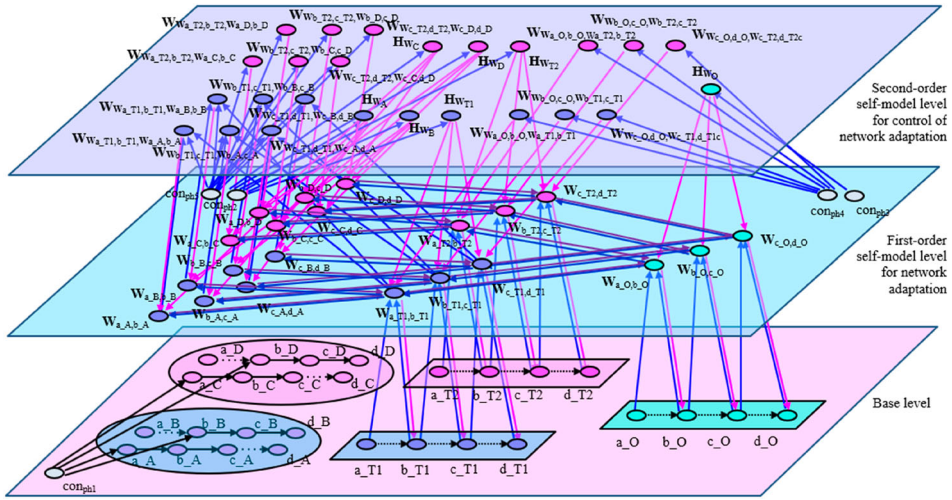
Figure 4. Example of an adaptive network model for organizational learning.
