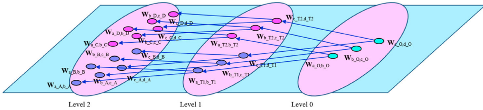
Figure 6. Only feedback learning. Each \underline{W} -state is by itself a strongly connected component as singleton. The \underline{W} -states of O form stratification level 0, the \underline{W} -states of the two teams T1 and T2 form level 1, and the \underline{W} -states of the four persons A to D form level 2.
