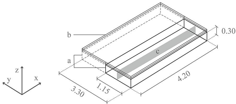
Fig. 2. Design strategies for redundancy and safety: (a) Division into two individual components (b) Float glass sheets (c) Design domain \Omega_{des} .
