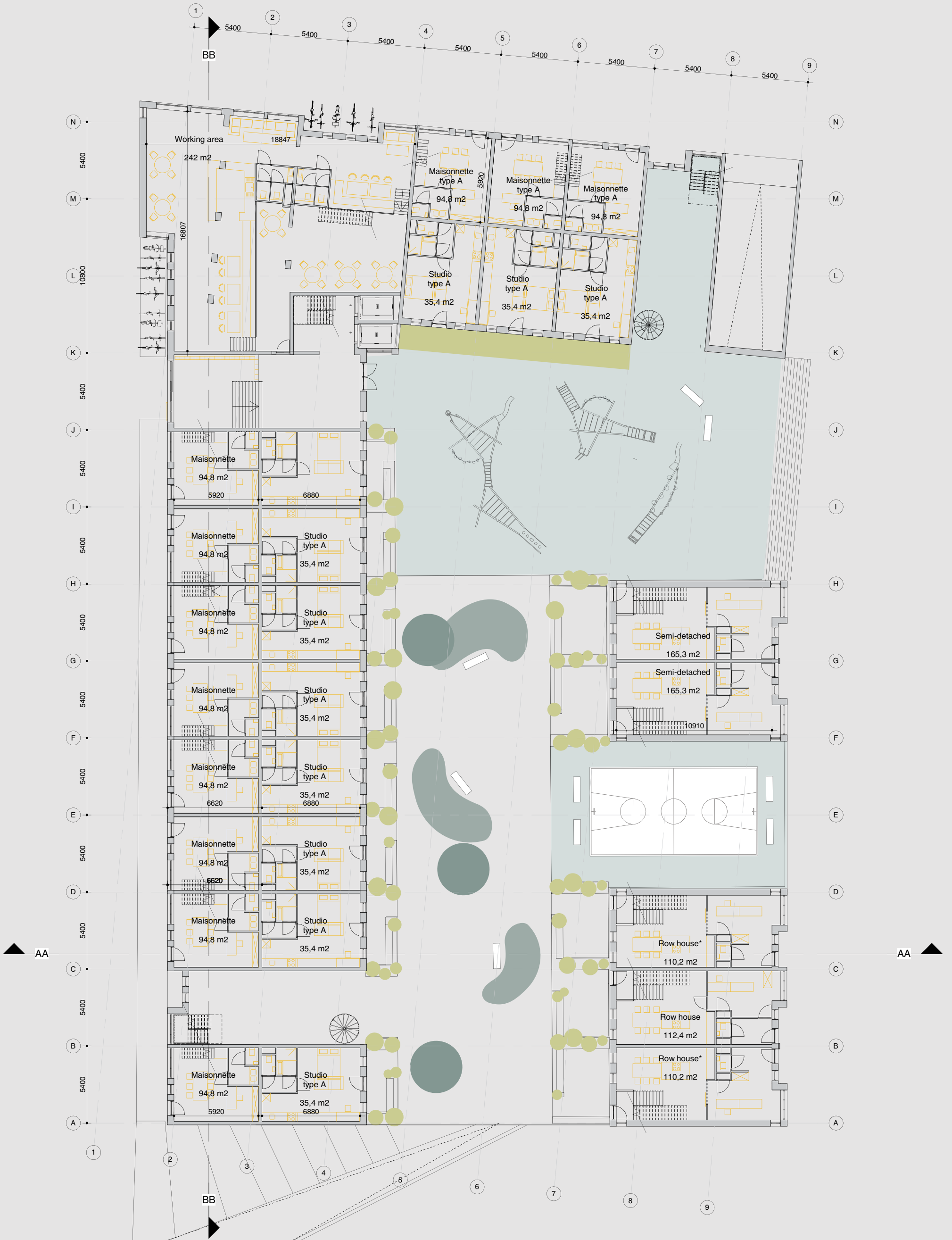
GROUND FLOOR SCALE 1:250
