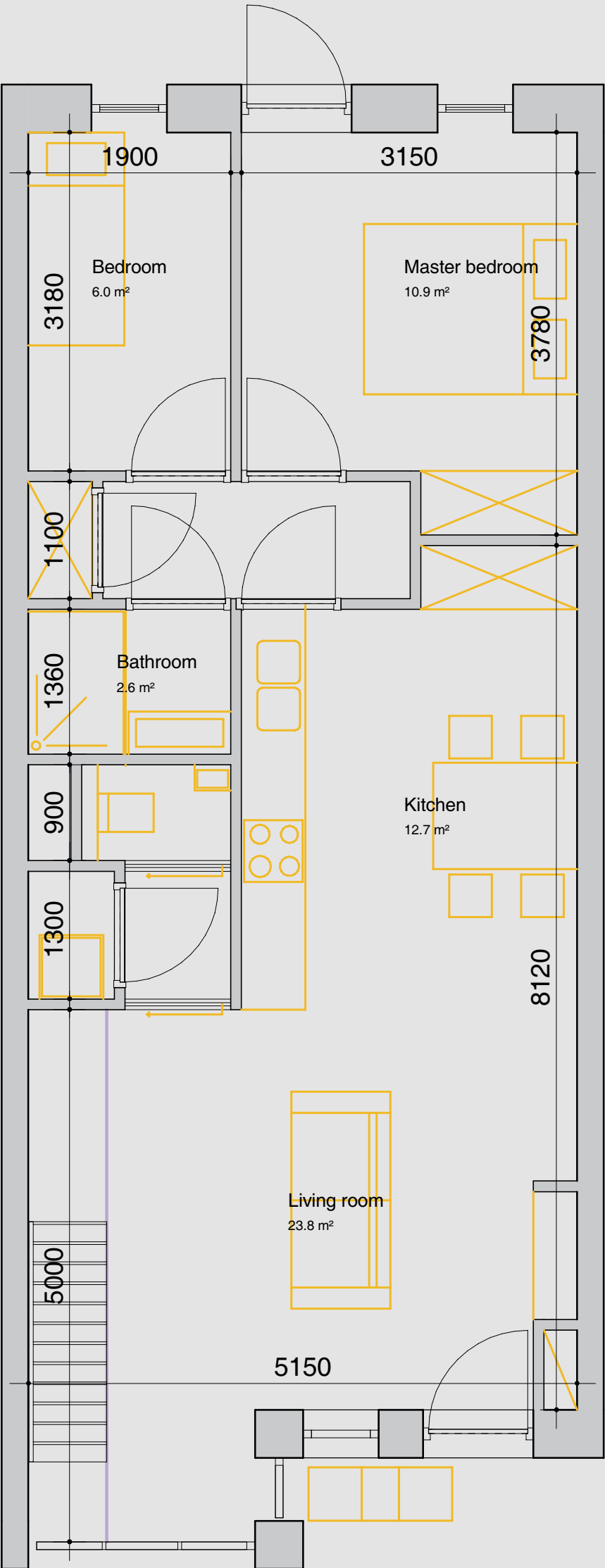
FIRST FLOOR
