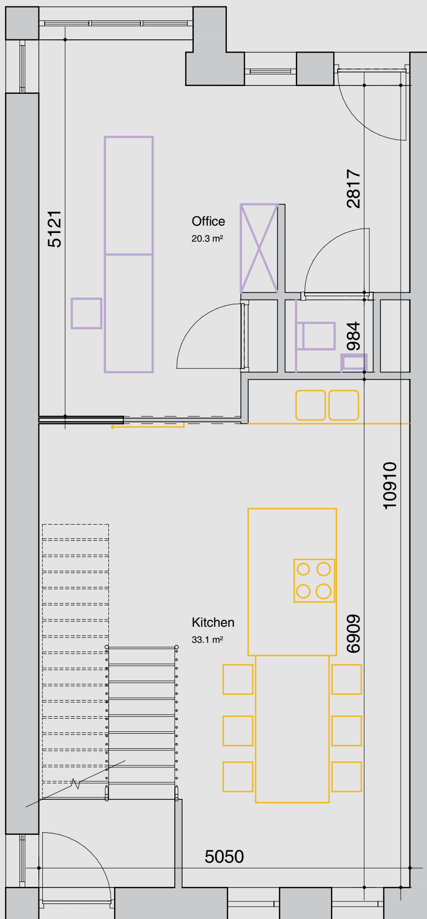
GROUND FLOOR
