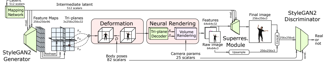
Figure 2: Illustration of the GNARF pipeline, including the StyleGAN2 generator, the tri-plane feature representation, feature volume deformation, neural volume rendering, image super-resolution as well as camera view and body-pose conditioned dual discrimination. The resolution of intermediate data and the final image is indicated for experiments with the AIST++ dataset.
