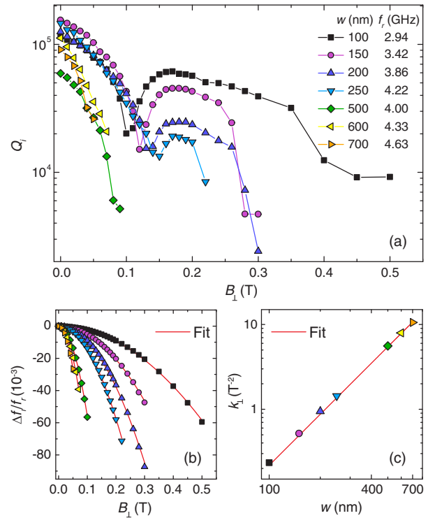
FIG. 4. Evolution of nanowire resonator characteristics with a perpendicular magnetic field, B_{\perp} . (a) Q_i as a function of B_{\perp} for various nanowire widths w . The dips in Q_i at low field suggest coupling to magnetic impurities, similar to the case for B_{\parallel} in Fig. 2. The narrowest resonator retains Q_i > 3 \times 10^4 up to B_{\perp} = 350 mT. (b) Fractional shift of the resonance frequencies with B_{\perp} . Same symbols as in (a). The red curves are best fits of \Delta f_r/f_r = -k_{\perp}(w)B_{\perp}^2 to the data. (c) Best-fit coefficient k_{\perp} versus w and best quadratic fit.
