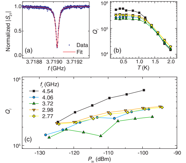
FIG. 2. Power and temperature dependence of intrinsic quality factors of five nanowire resonators. (a) Normalized absolute transmission around a typical resonance. The curve is constructed from the best fit to the complex-valued feedline transmission data [16,28]. (b) Temperature dependence of intrinsic quality factors measured at a fixed input power P_{\text{in}} \approx -110 dBm. The symbols correspond to the legend in (c). Two distinct regimes are observed for T < 1 K and T > 1 K, in which dominant loss is expected from TLS and quasiparticle dissipation, respectively. (c) Power dependence of intrinsic quality factors measured at 280 mK. The positive slope is consistent with TLS-dominated loss.
