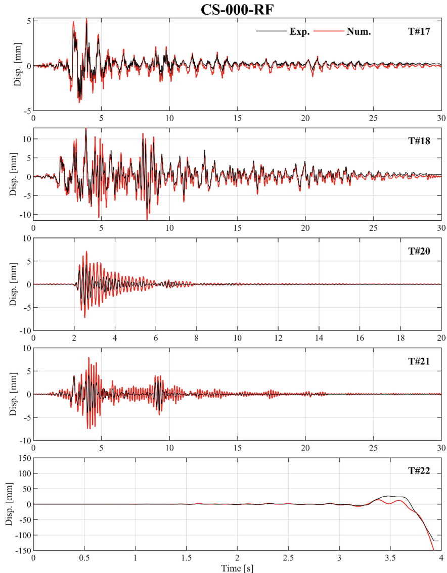
Fig. 4. Comparison of numerical and experimental displacement time histories for wall CS-000-RF
