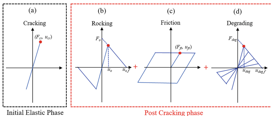
Fig. 2. Schematic representation of the proposed model.
