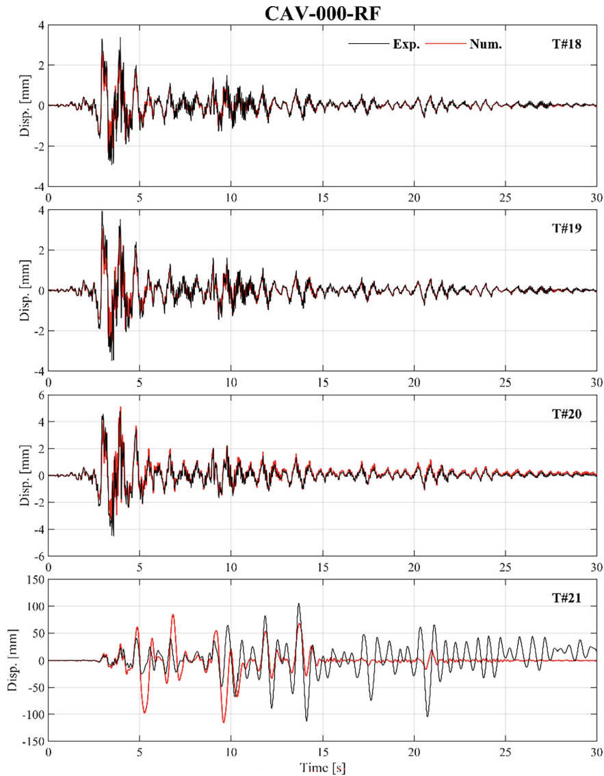
Fig. 6. Comparison of numerical and experimental displacement time histories for wall CAV-000-RF
