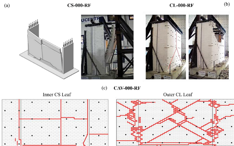
Fig. 1. Failure mechanisms of walls (a) CS-000-RF; (b) CL-000-RF and (c) CAV-000-RF observed experimentally.
