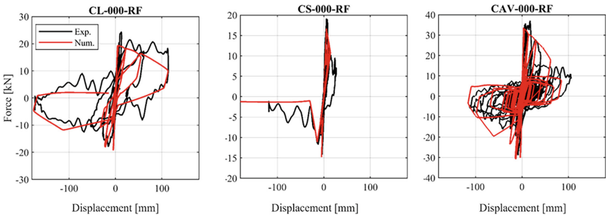
Fig. 3. Comparison of numerical and experimental force-displacement hysteresis.
