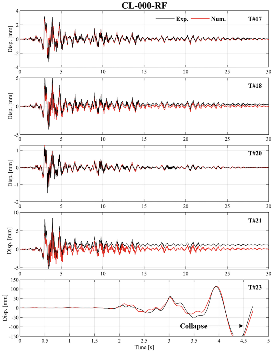
Fig. 5. Comparison of numerical and experimental displacement time histories for wall CL-000-RF
