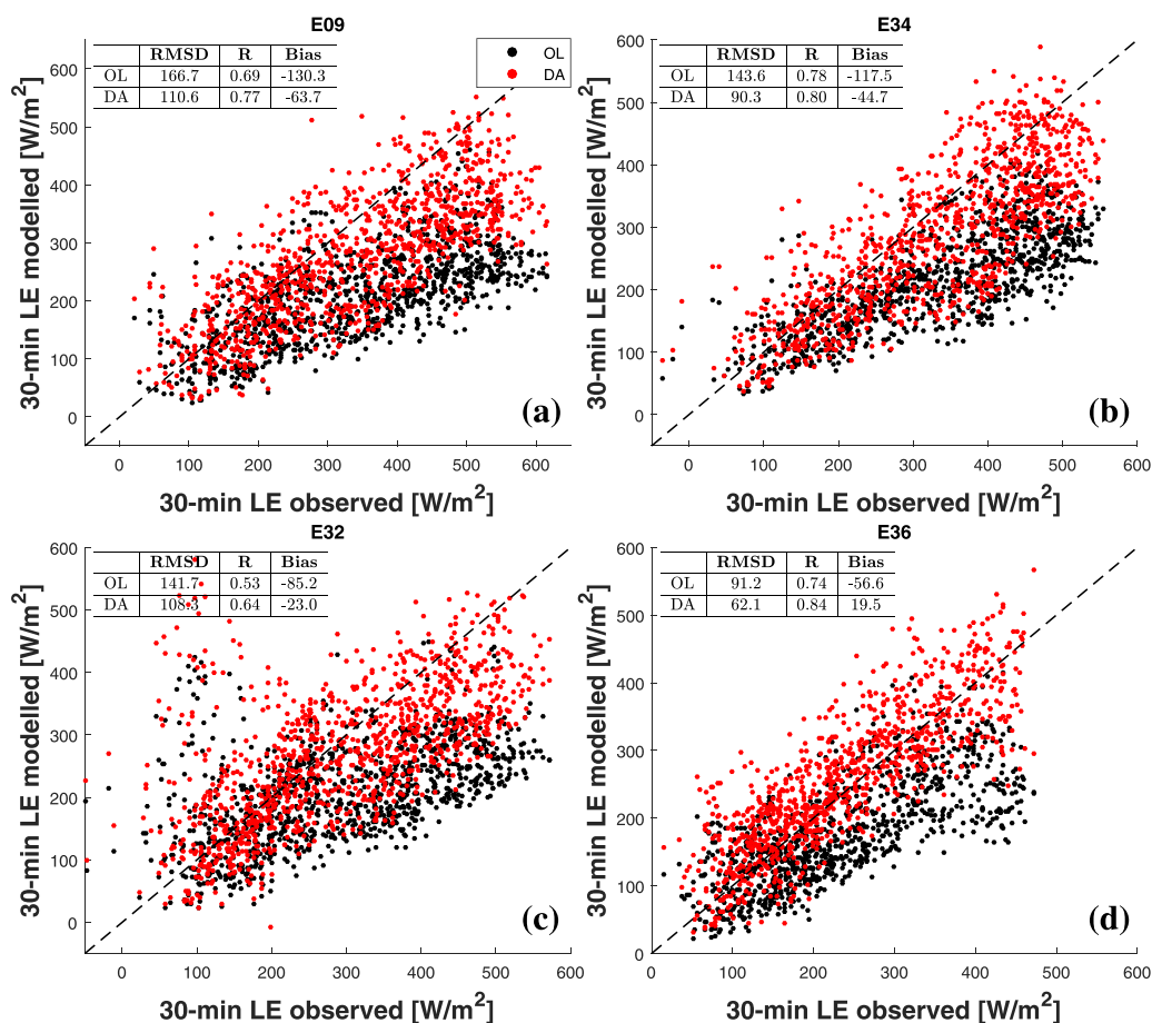
Figure 7. As in Figure 6 but for 30 min LE estimates.
