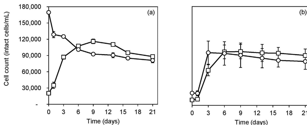
Fig. 4. Examples of bacterial growth curves in pasteurized (—□—) and non-pasteurized (—○—) site-Remin samples analyzed on two different dates: (a) with fresh calcite grains ( C_{0, \text{non-pasteurized}} > C_{\text{max}} ) and (b) when the calcite contactors have been in operation for several weeks ( C_{0, \text{non-pasteurized}} < C_{\text{max}} ). Each sample was inoculated with CTW. Error bars represent the standard deviation of triplicate measurements.
