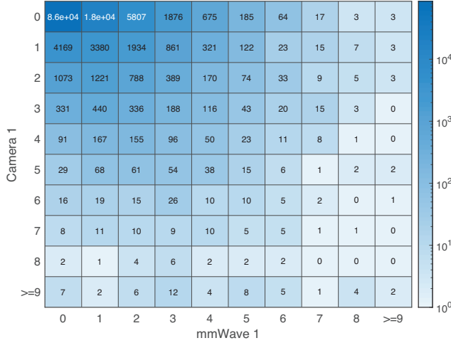
Fig. 6: Confusion matrix. The heatmap follows a log scale.
