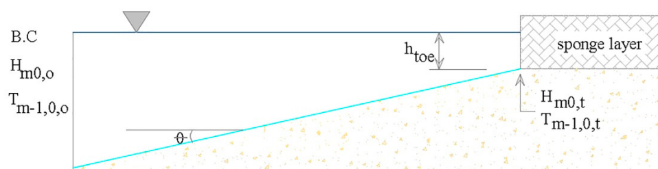
Figure 3. Wave parameters at toes in SWASH model for case studies.
