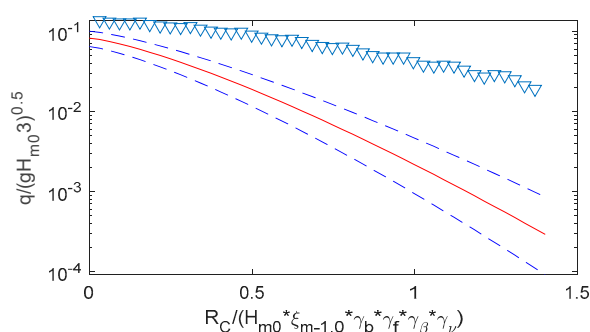
Figure 12. Comparison to Altomare [5] (red solid line: prediction using mean value approach of Altomare; dashed line: \pm 1.64\sigma ; and triangle: SWASH values).
