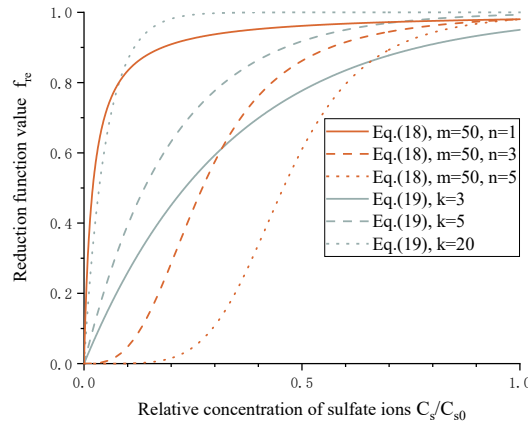
Fig. 5. Reduction functions with different forms and parameters.
