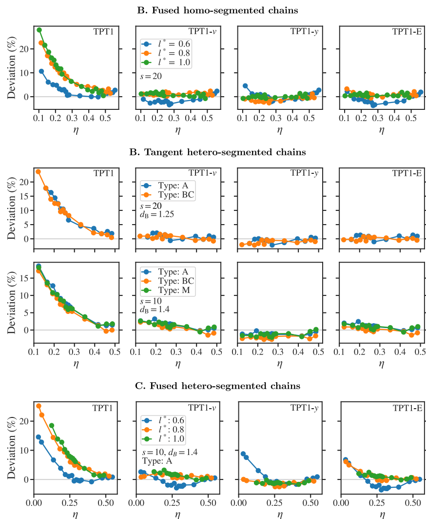
FIG. 5. Percentage deviations of TPT1, TPT1-v, TPT1-y, and TPT1-E with respect to molecular simulation data for the residual pressure p^{\text{res}} = p - p^{\text{ig}} of (a) fused homo-segmented hard-sphere chains of 20 segments, (b) tangent hetero-segmented hard-sphere chains of 10 and 20 segments, and (c) fused hetero-segmented hard-sphere chains of 10 segments. Type BC denotes a block-copolymer with s/2 segments of diameter d_A = 1 , followed by s/2 segments of diameter d_B ; type A denotes a chain of alternating type A and type B segments; and type M denotes an equimolar mixture of chains with type A segments and chains with type B segments.
