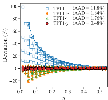
FIG. 4. Percentage deviation of TPT1, TPT-E, TPT1- v , and TPT1- \gamma with respect to molecular simulation results for the residual pressure p^{\text{res}} = p - p^{\text{ig}} (with p^{\text{ig}} = \rho k_B T ) of homo-segmented tangent hard-sphere chain fluids comprising between two and 500 hard spheres per molecule. 35,61,77 Lines act as a guide for the eye for chains of 201 and 500 segments.
