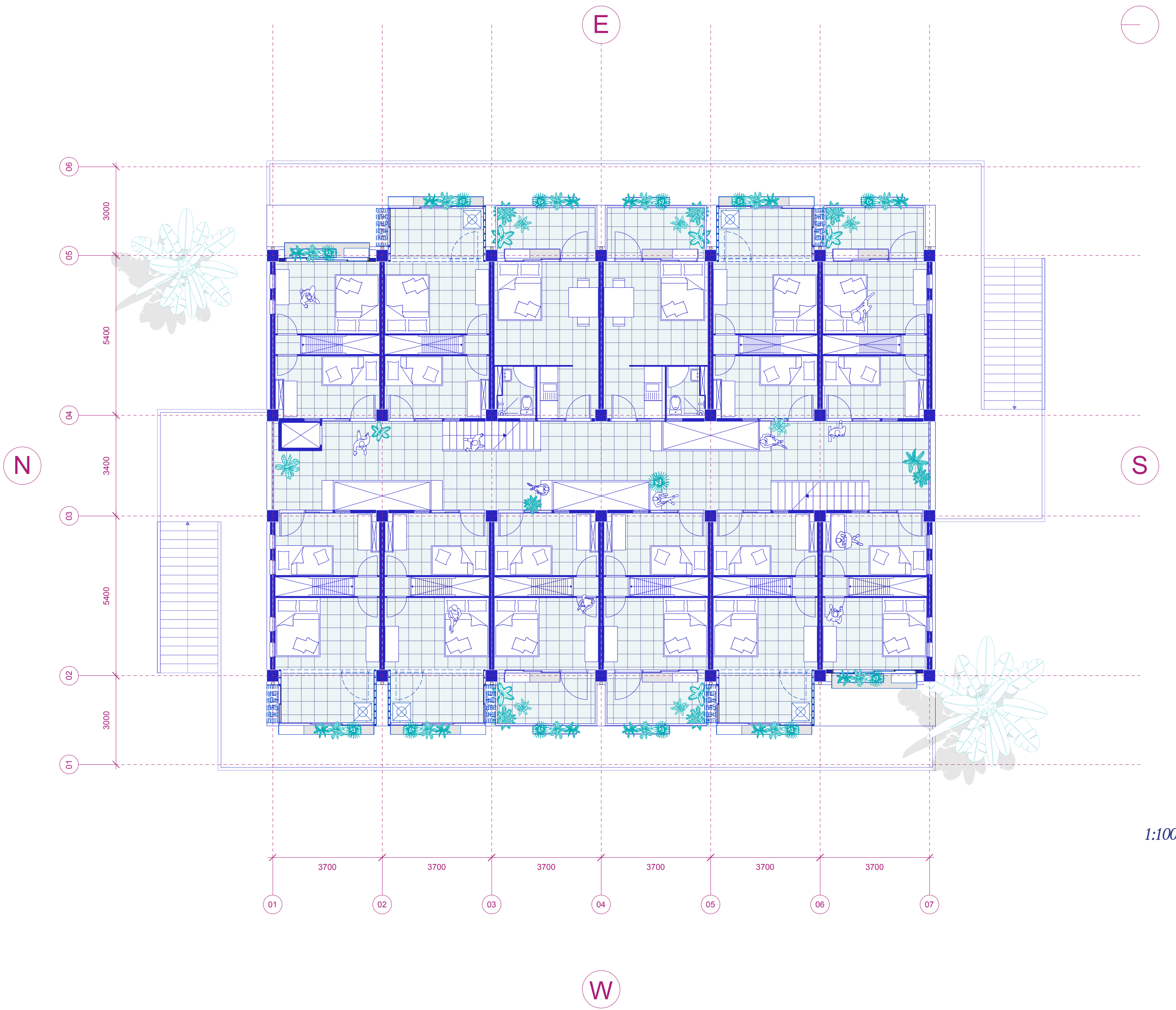
FLOORPLANS +0
