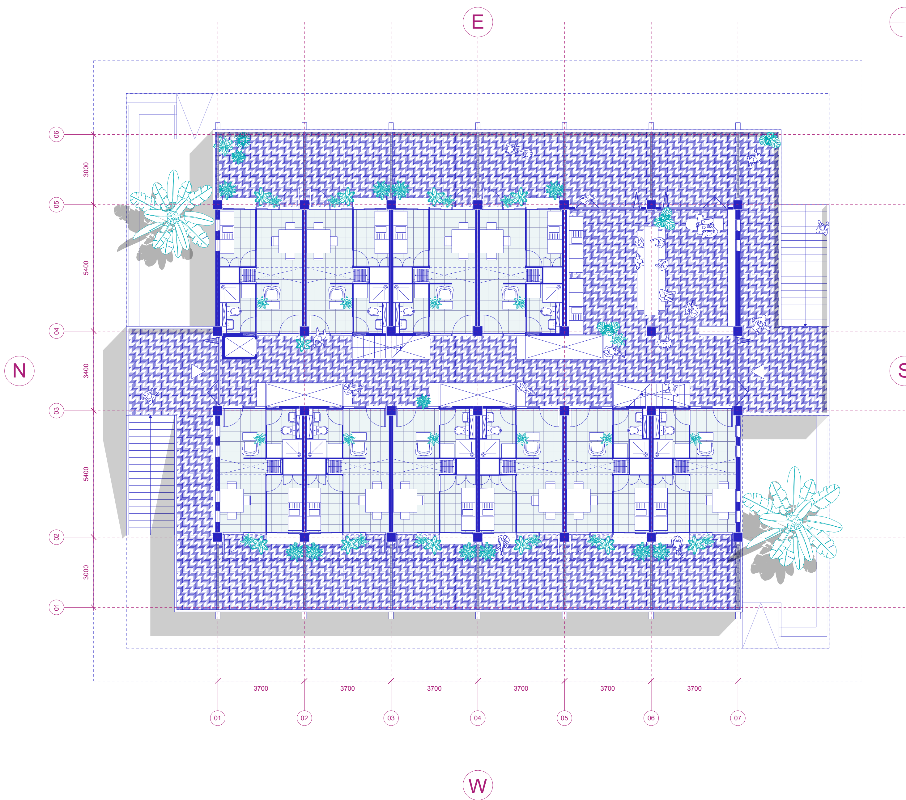
FLOORPLANS +1
