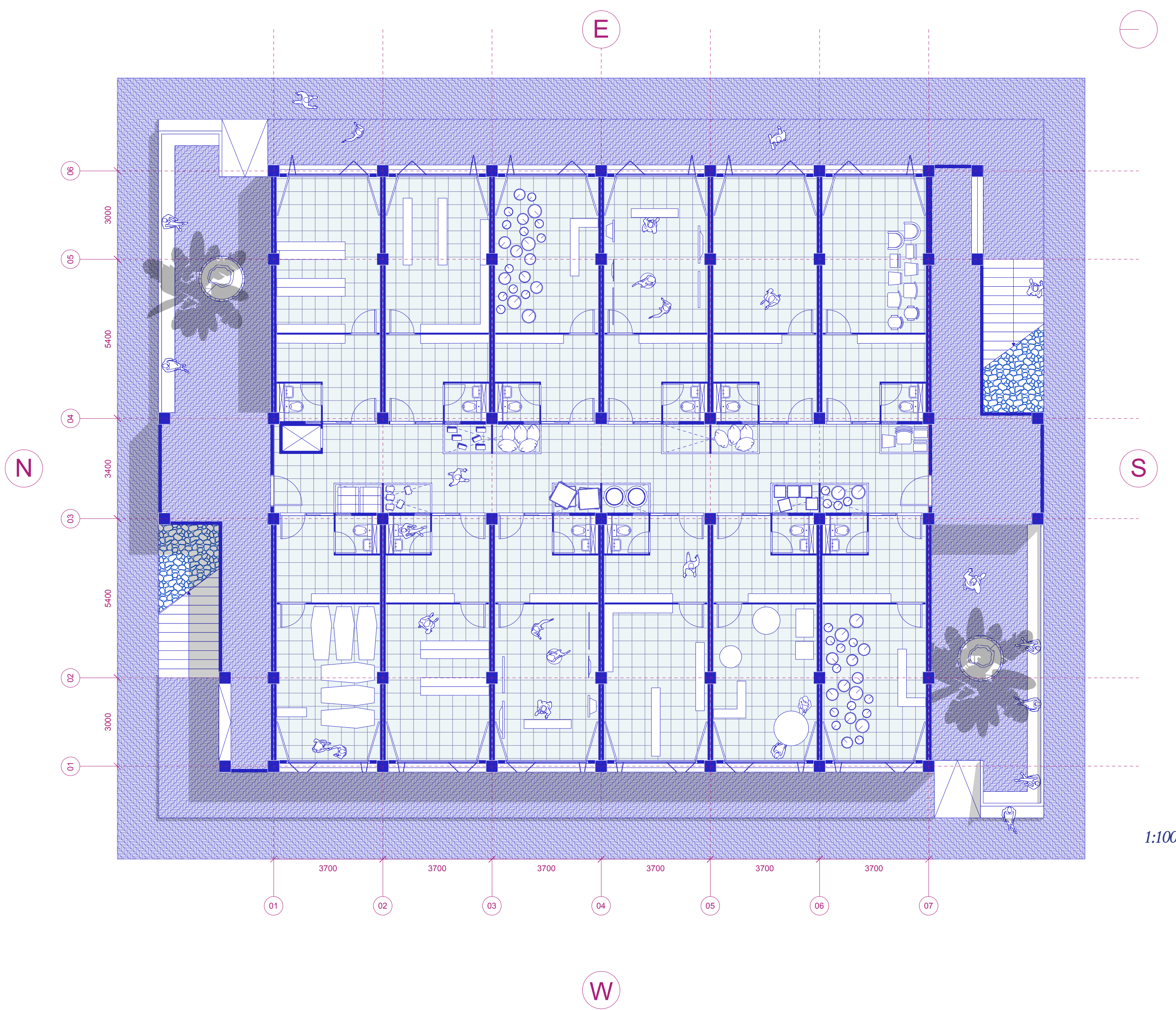
FLOORPLANS +0
