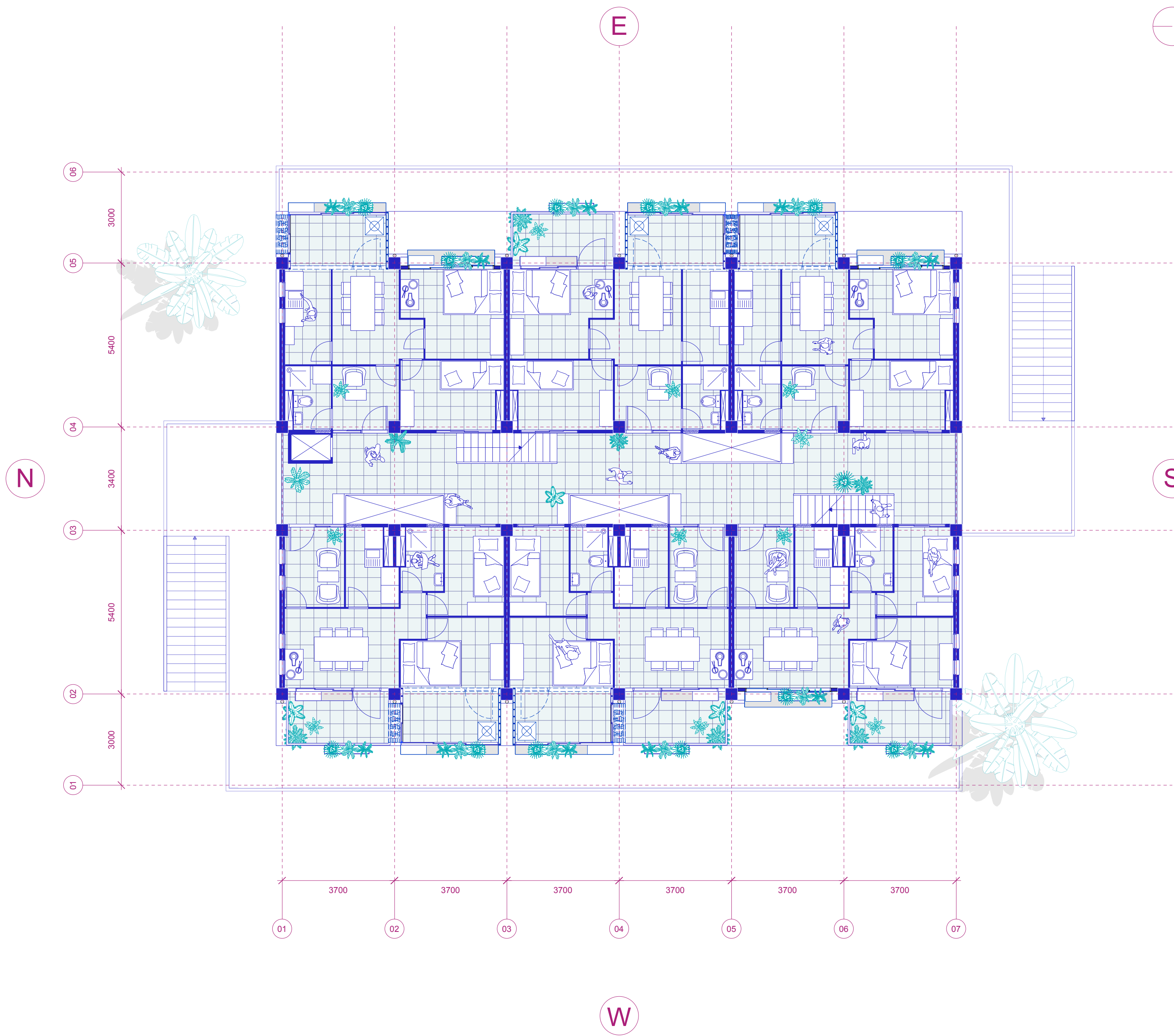
FLOORPLANS +1
