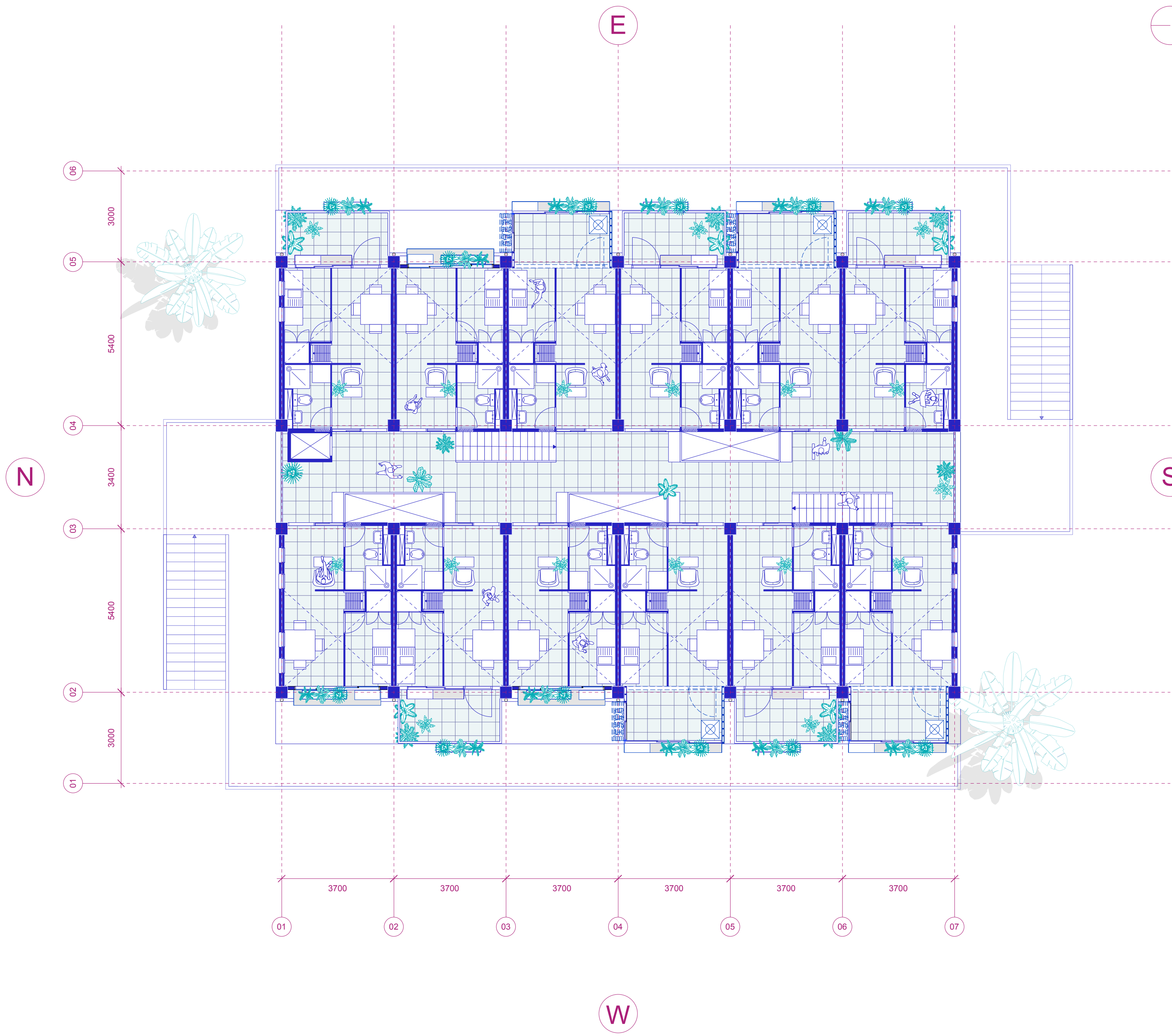
FLOORPLANS +5
