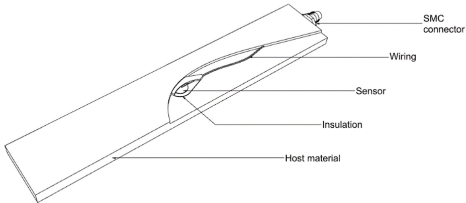
Fig. 6. Cut-through drawing of the test sample, showing different components.
