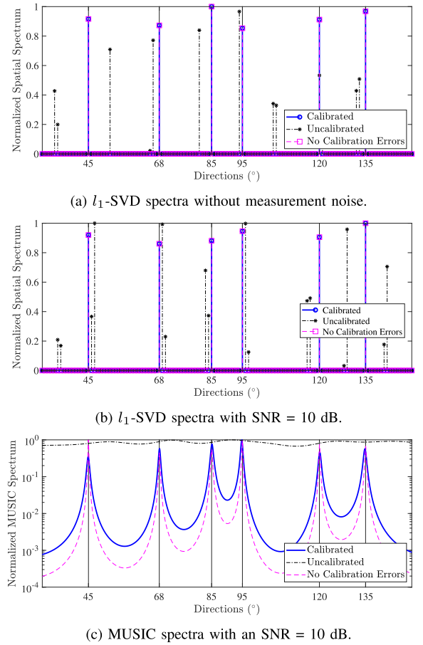
Fig. 1. The l_1 -SVD and MUSIC spectra using the element-space data model based solver in (22) for an AVS ULA with M = 8 , N = 6 and L = 50 . The true DOAs are indicated by the black solid lines.
