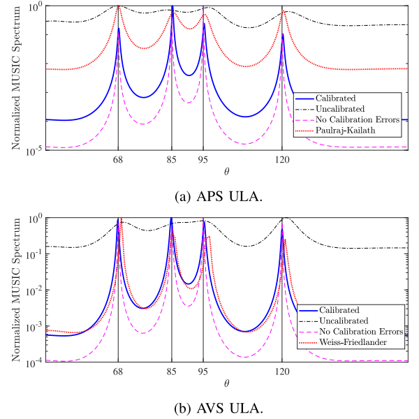
Fig. 3. The MUSIC spectra for both the APS and AVS ULA based on the co-array data model solver in (27) with L = 1000 , \text{SNR} = 10 dB, M = 8 and N = 4 far-field sources. The true DOAs are indicated by the black solid lines.
