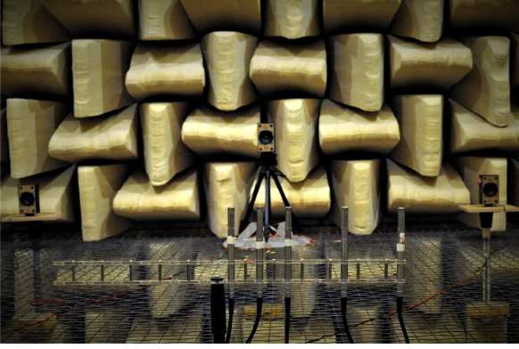
Fig. 10. Picture of the experimental setup considering five AVSs and three speakers, located at a radius of r = 3.6 m.
