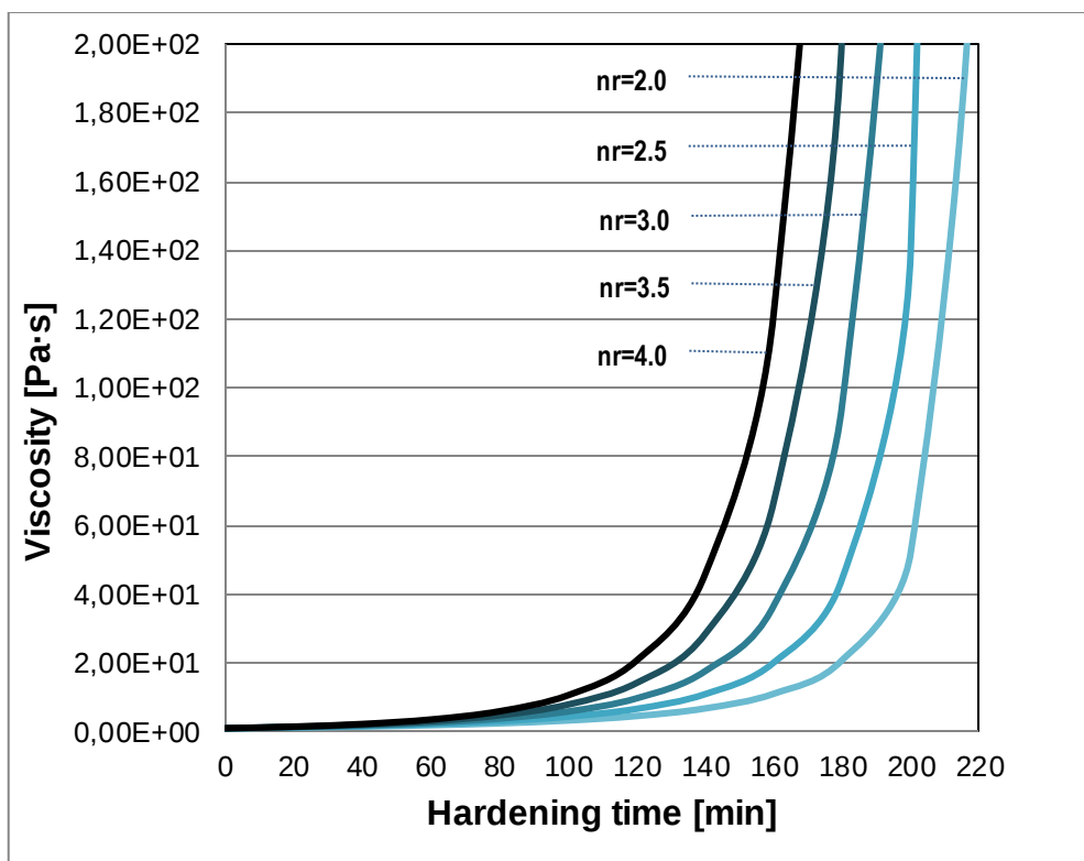
FIGURE 7 Predicted viscosity development of epoxy modified bitumen under isothermal heating conditions for different n_r at T=100\text{ }^{\circ}\text{C} ( E_a=50\text{ kJ/mol} , n=0.2 , k_0=100\text{ 1/s} , \alpha_g=0.6 )
