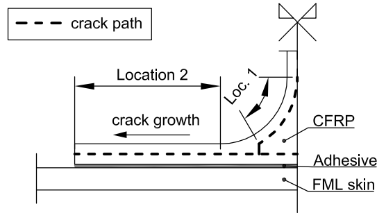
Figure 10: Locations of the fractographic analysis along the crack path.
