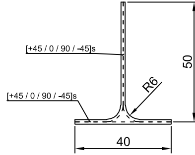
Figure 1: CFRP Stiffeners' configuration (dimension in mm).
