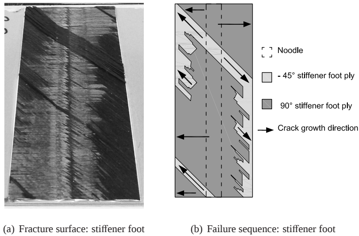
Figure 5: Typical fracture surfaces and failure sequence for static loading under the complete temperature range ( -55^{\circ}\text{C} up to +100^{\circ}\text{C} ).
