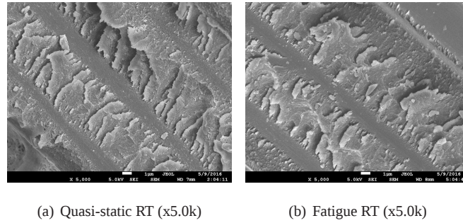
Figure 11: Fracture surface at Location 2: crack propagation at the fibre imprint side
