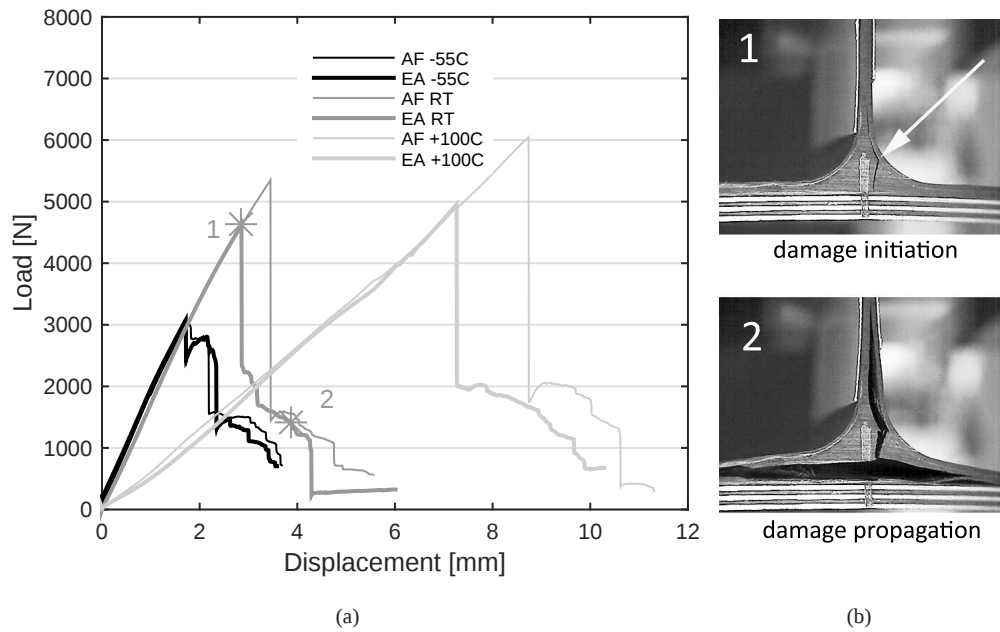
Figure 4: Typical load-displacement curves at the three temperatures tested for the two adhesives (a) and correspondent failure sequence for EA9696 RT test series (b) (the grey line crossing the stiffener noodle and the FML skin was drawn with a pen marker to identify the middle of the specimen).
