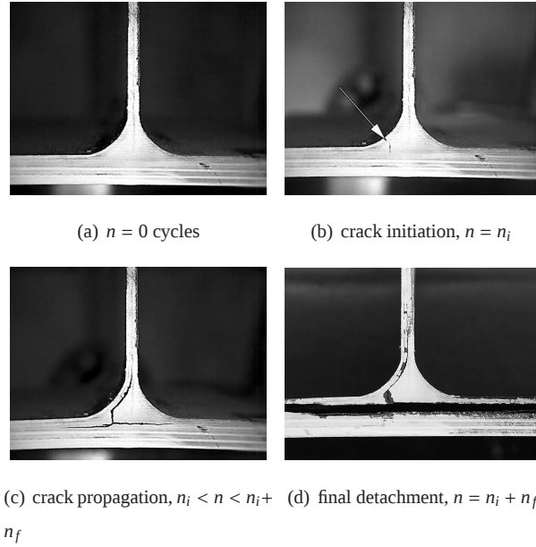
Figure 7: Typical fatigue damage events ( n –number of fatigue cycles; n_i – number of cycles to crack initiation – fatigue life initiation ; n_f – number of cycles from crack initiation to complete detachment – fatigue life propagation ).
