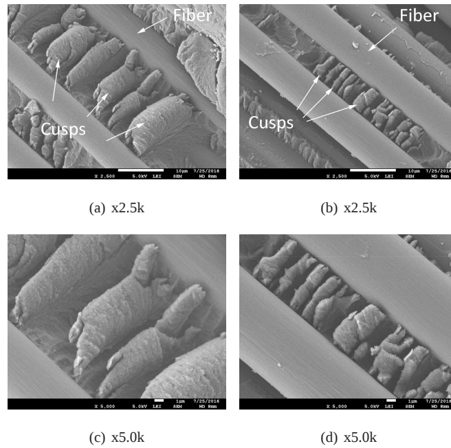
Figure 12: Fatigue fracture surfaces at Location 2: crack propagation, at the fibre side – stiffener foot plies.
