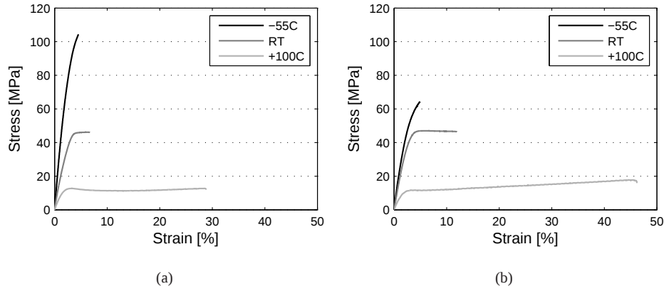
Figure 3: Tensile stress-strain curves of adhesive (a) AF163-2 and (b) EA9696.
