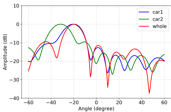
Figure 5.10: Beamforming results
