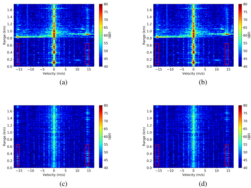
Figure B.6: Range-Doppler map of (a) contentional autocorrelation, (b) compensational autocorrelation, (c) conventional cross-correlation and (d) compensated cross-correlation
