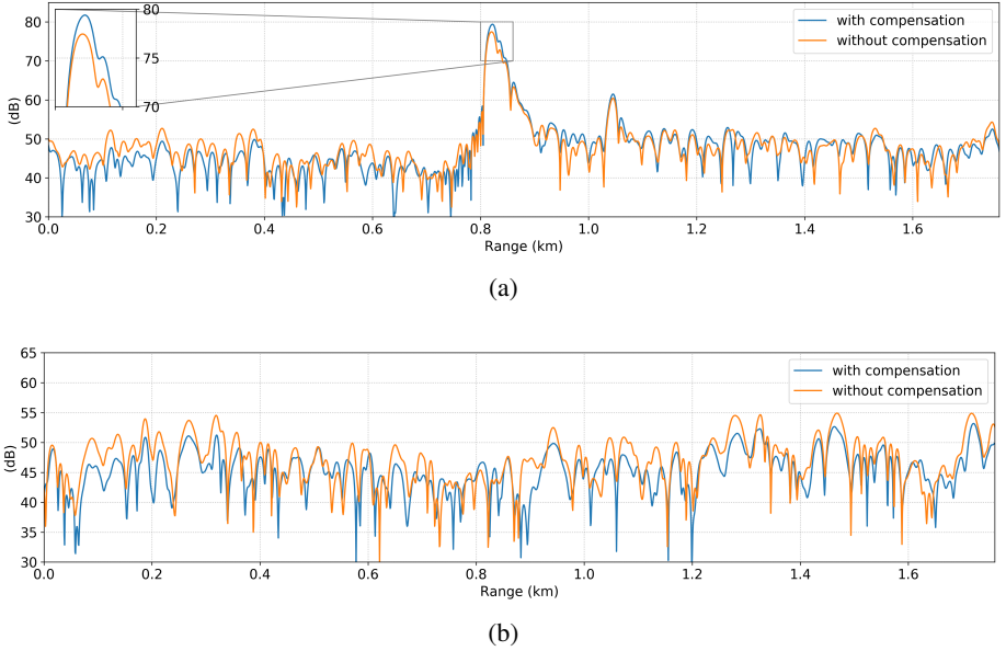
Figure B.7: Range-Doppler map slicings at v = -15.65 m/s of (a) autocorrelation and (b) cross-correlation.
