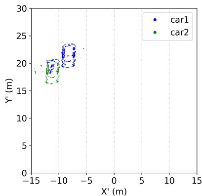
Figure 5.11: Reconstructed Scene
