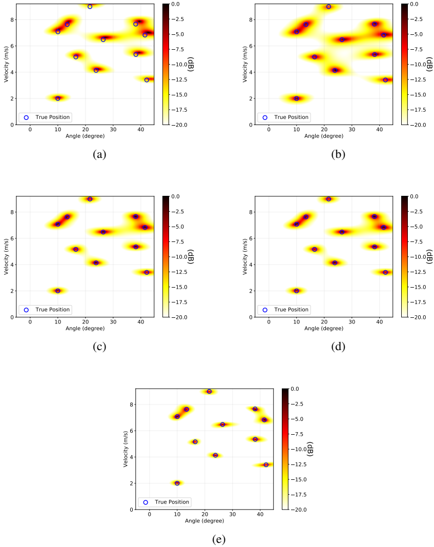
Figure 3.9: Angle-Velocity maps of B = 4 GHz and \text{SNR} = 20 dB for (a) 2D MUSIC without phase compensation, (b) 2D MUSIC after Keystone transform, (c) 2D MUSIC with phase compensation and accelerated by Lanczos algorithm, (d) 2D MUSIC with phase compensation and accelerated by Rayleigh-Ritz step and (e) 2D MUSIC with phase compensation and accelerated by inverse algorithm
