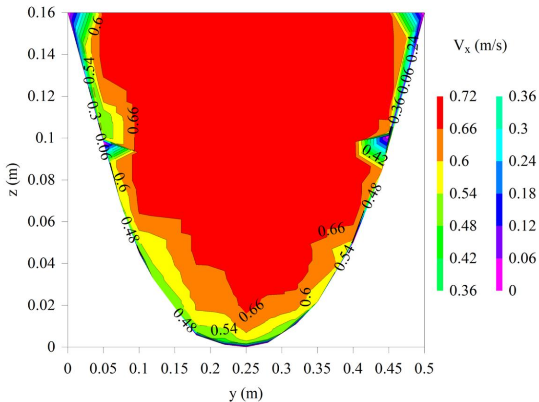
F03B_Contour 35lps x=7.15m UPDATED
