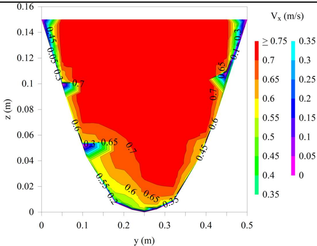
F03A_Contour 35lps x=2M UPDATED
