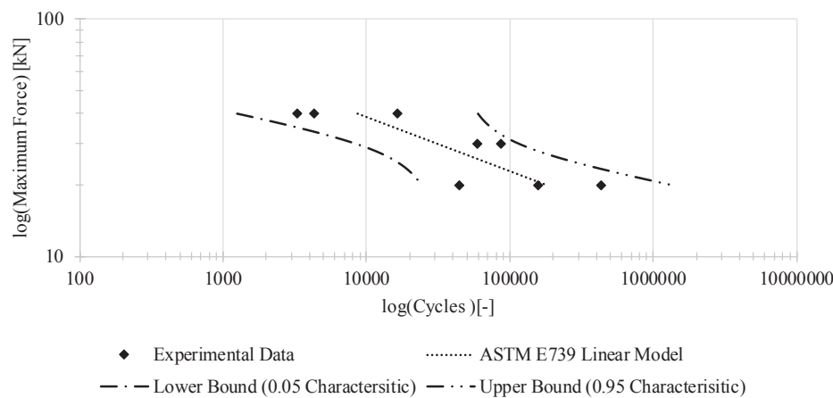
Fig. 10. ASTM E739 statistical analysis.
