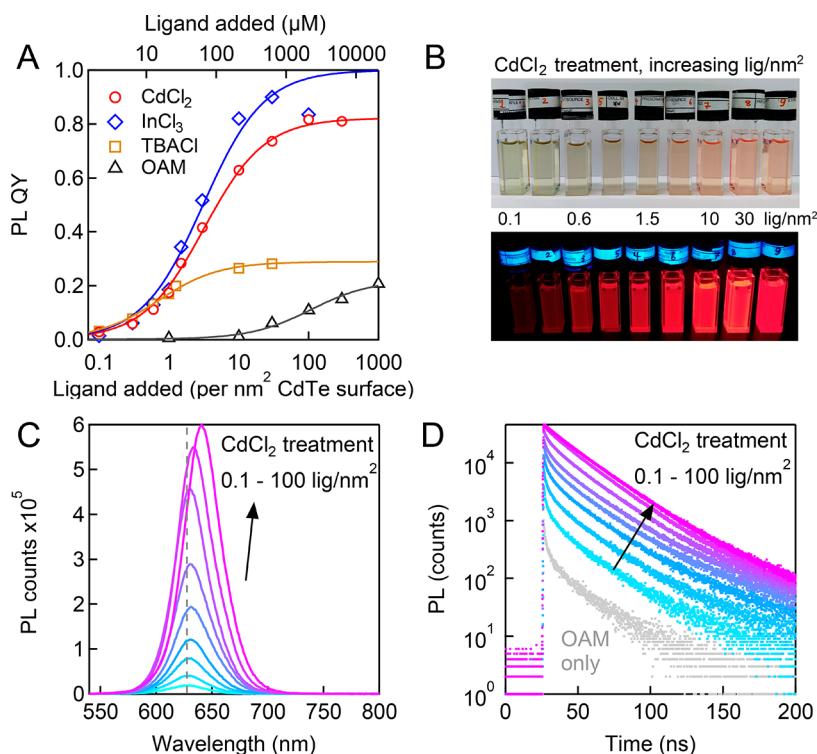
Figure 4. Effect of ligand concentration on CdTe QDs (3.8 nm, 0.456 \mu\text{mol}/\text{L} in toluene) after treatment at 95 ^{\circ}\text{C} for 15 min with CdCl 2 , InCl 3 , TBACl (9 equiv of OAM), and OAM only ligand. (A) PL QY of CdTe QDs after treatment with ligands as a function of concentration of added ligand per \text{nm}^2 of total CdTe surface area. Top axis shows the final ligand concentration in the solution. Lines are fits using eq 7 (see text). (B) Photographs under ambient room light (top) and UV light (bottom) showing effect of CdCl 2 treatment at increasing CdCl 2 concentrations (in \text{nm}^{-2} ) on QD PL. (C) PL spectra of CdCl 2 -treated QDs at increasing amounts of ligand added from 0.1 to 100 \text{lig}/\text{nm}^2 . Dashed gray line shows position of PL peak before treatment. (D) PL decay curves of CdCl 2 -treated QDs as a function of ligand concentration.
