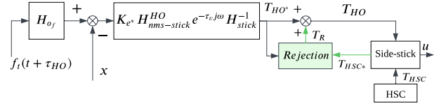
Fig. 7: Torque rejection model
