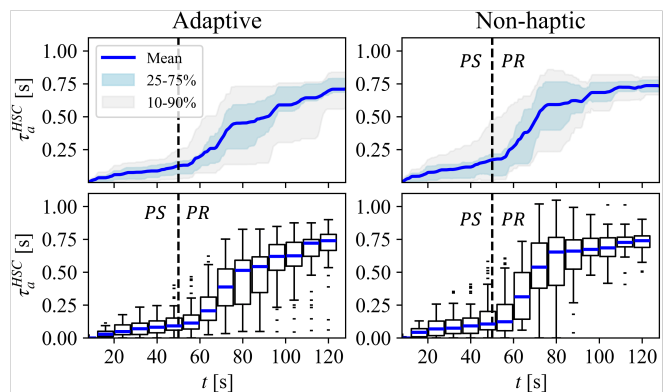
Fig. 24: Experiment adaptive look-ahead time (PS-PR)
