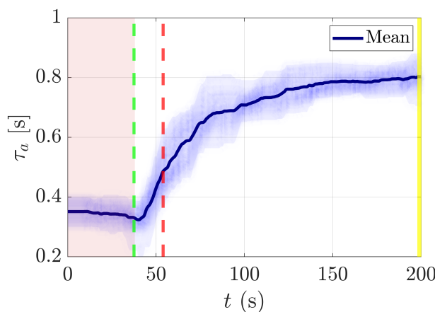
Figure 3.46: XC-AHSC reversed adaptive look-ahead time, N=100
