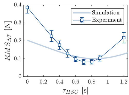
Figure 2.12: Conflict torque [6]
