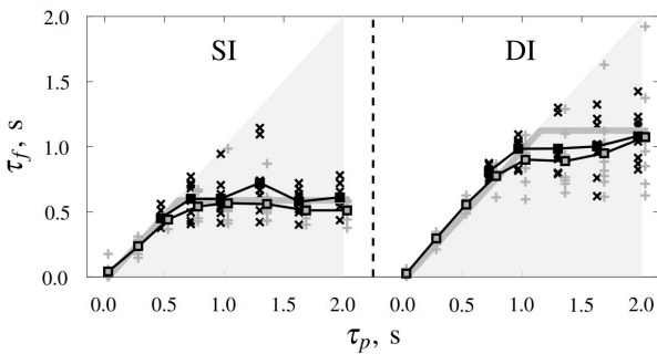
Figure 2.3: Look-ahead time adaptation [13]
