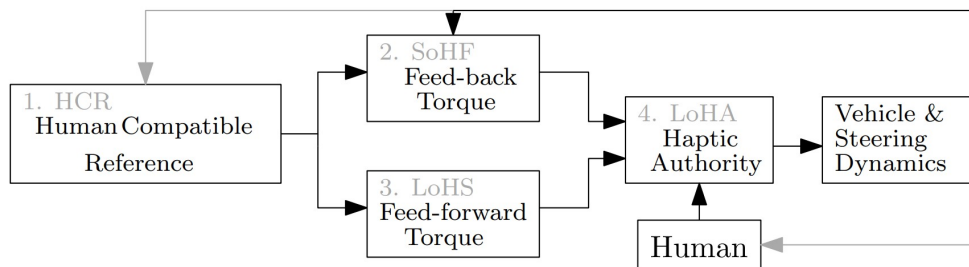
Figure 2.5: FDCA design philosophy [16]
