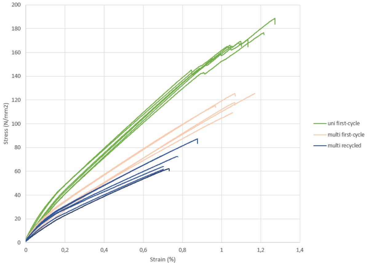
Figure 1: Tensile test results
