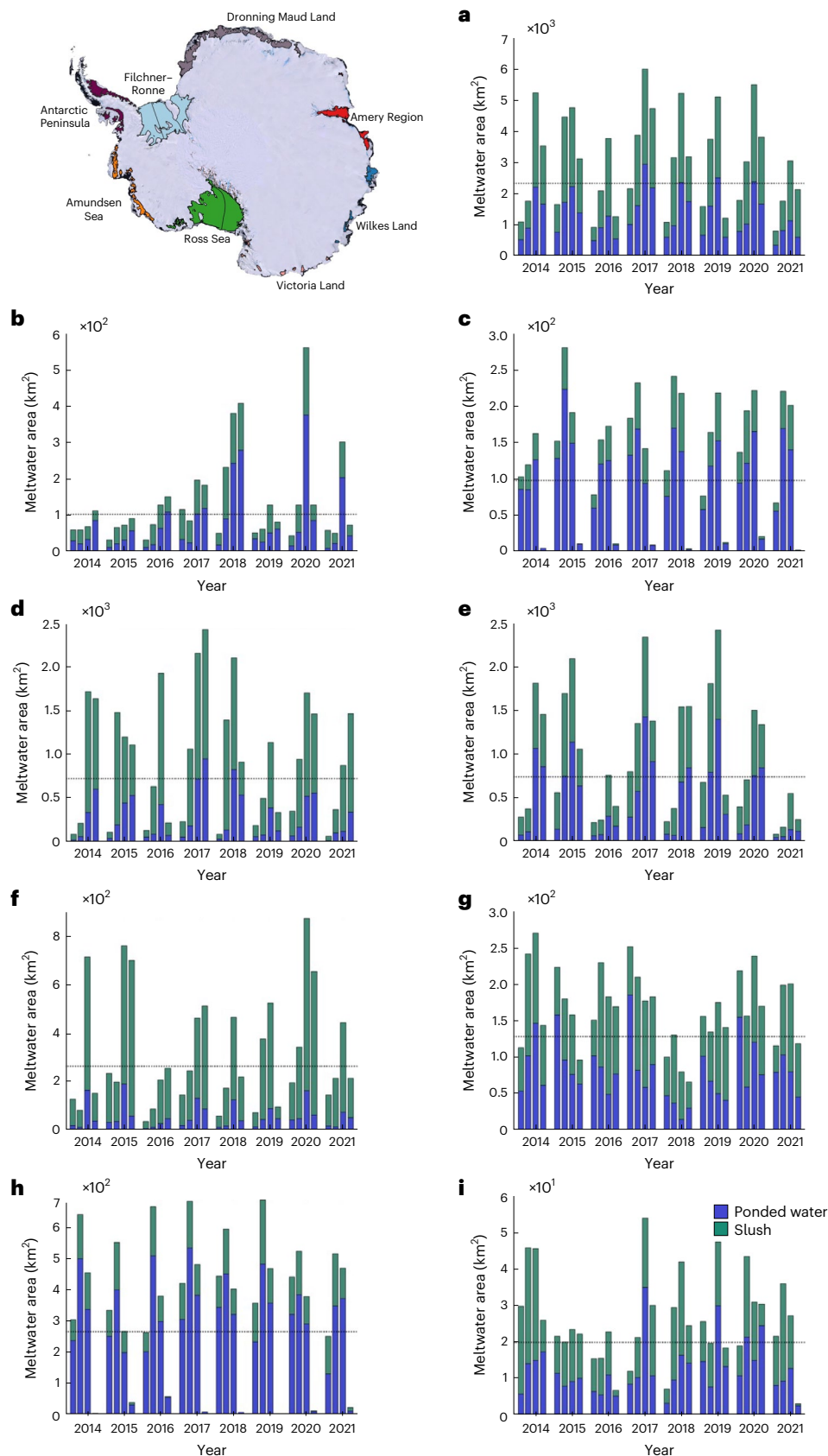
Fig. 1 | Total surface meltwater area, total ponded water area and total slush area. a–i, Summed data for all ice shelves on the continent ( a ), the Antarctic Peninsula ( b ); the Filchner–Ronne Region ( c ); Dronning Maud Land ( d ); the Amery Region ( e ); Wilkes Land ( f ); Victoria Land ( g ); the Ross Sea Region ( h ); and the Amundsen Sea Region ( i ). For each year, bars represent, from left to right, monthly data from November, December, January and February. Stacked bars are
