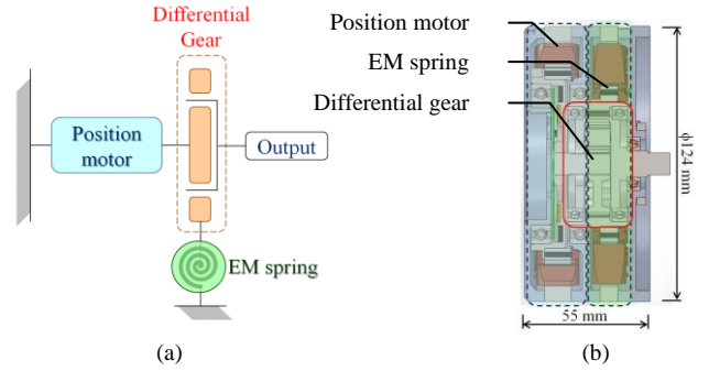
Fig. 3 EM spring VSA design. (a) Connection between components. (b) Component arrangement and structure design.
