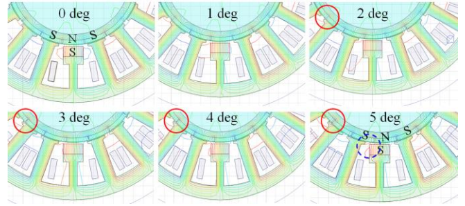
Fig. 6 Simulation results of magnetic flux flow at different angle (Type 1 EM spring at a current of 10.5A). The red circle indicates that a local flux loop occurred at the edge of the tooth. The blue dotted circle indicates the flux distortion around the edge of the magnet.
