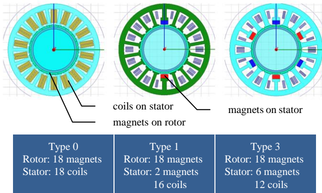
Fig. 2 Three EM spring module arrangements.
