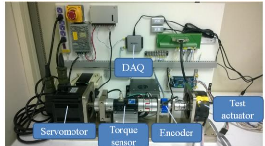
Fig. 4 Experimental setup
