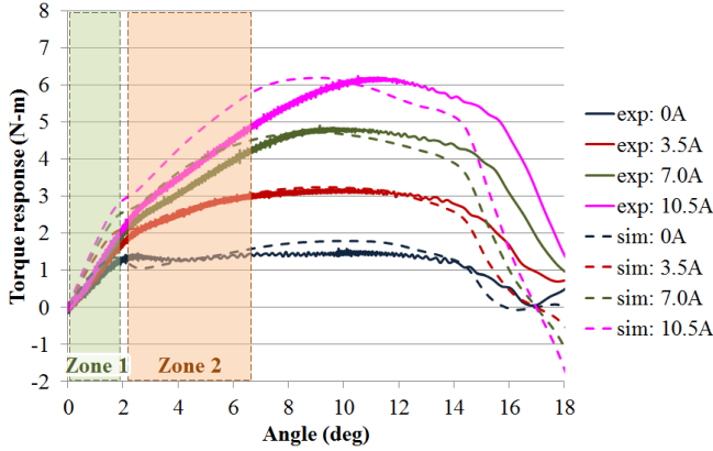
Fig. 5 Experiment (solid lines) and simulation results (dotted lines) of the ramping force test at different currents (Type 1 EM spring). The green shaded region, zone 1 covers the first linear section of the torque response; the brown region, zone 2, covers the second linear region of the response curve.
