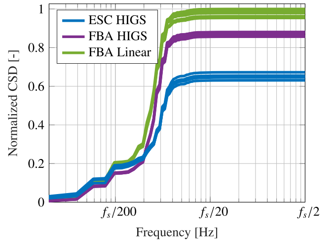
Fig. 13. Cumulative energy spectral density of the error of the five motions of the different controllers, with the FBA-tuned HIGS-based controller (FBA HIGS), FBA-tuned linear controller (FBA linear) and the ESC-tuned HIGS-based controller (ESC HIGS).
