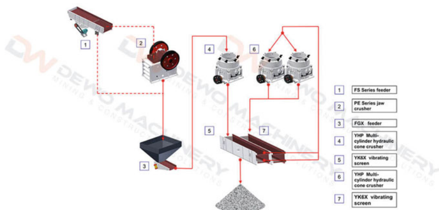
Fig. 1 Process of steel slag production [13]
