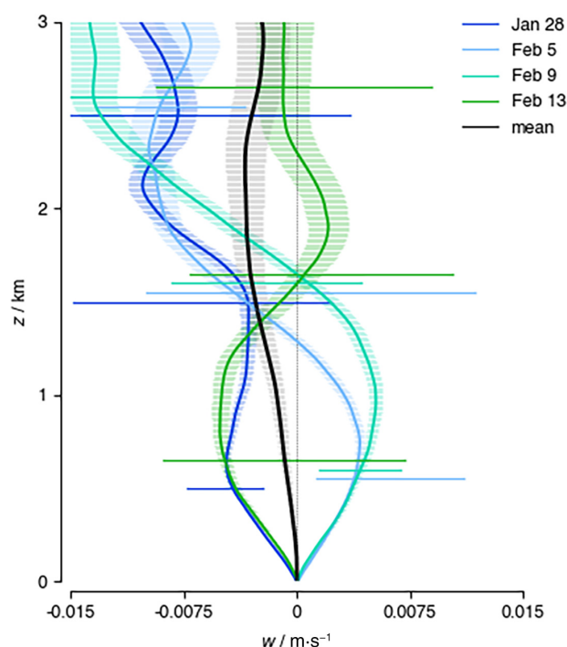
FIGURE 9 Flight-mean vertical velocity profile on January 28, February 5, February 9, and February 13, and as the EUREC4A/ATOMIC flight mean (in black). The shaded area corresponds to the mean residual standard error (Equation 2) and horizontal lines at selected heights span the minimum and maximum w encountered on a flight. On February 5 and February 9, mean rising motion at low levels and descending motion aloft coincide with the layer of positive F_s above z = 1.5 km seen in Figure 7c,d [Colour figure can be viewed at wileyonlinelibrary.com ]
