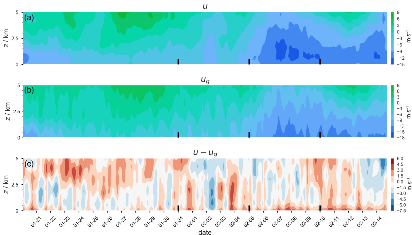
FIGURE 3 Evolution of u , u_g , and the geostrophic departure u - u_g from ERA5 reanalysis over a 1,000 \times 1,000 \text{ km}^2 area, illustrating that, while u follows u_g on synoptic time-scales, significant departures from geostrophy are present on (sub-)daily time-scales [Colour figure can be viewed at wileyonlinelibrary.com ]
