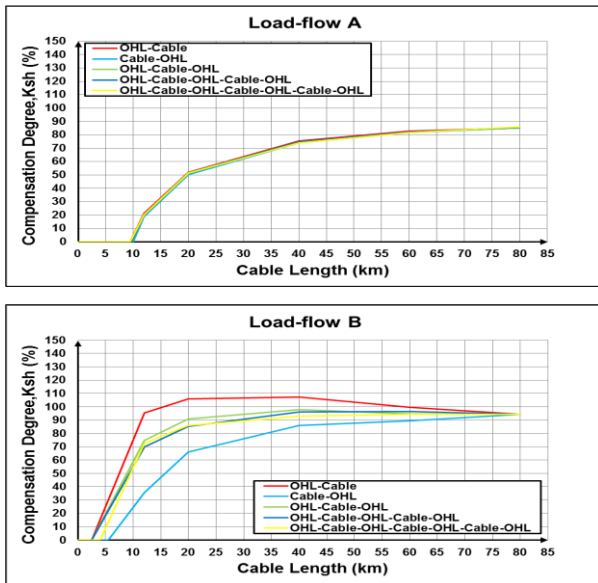
Figure 5: Minimum required shunt compensation degree vs. cable length for different mixed-line configurations during double-circuit operation.
