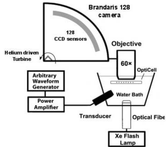
Fig. 5. Schematic of the optical setup used with the Brandaris 128 camera to optically record microbubble dynamics.
