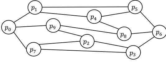
Fig. 1. A reliable communication graph with N = 10 and f = 1 .
