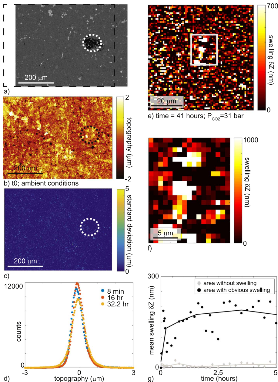
Fig. 8. Deformation of sample CO 2 _11, Pomeranian shale. The circles indicate the location of a patch of organic matter (black), interspersed with pyrite (bright), an area which is investigated in greater detail in Fig. 8e–g); a) backscattered electron image taken before completing sample assembly. The dotted rectangle indicates the approximate location of topography measurements shown in b) where the initial topography is measured with the white light interferometer; c) map with the standard deviation of each pixel through time. High numbers indicate the pixel moved in height during the experiment. In approximately the same location as where the organic matter was present in the SEM image (white circle) there are measurable topography changes; d) histogram of the height data at different times. There is a small change in the histogram shape, close to the measurement error of 200 nm. 8e–g) Close-up of the area containing organic matter; e) a 20 × 20 μm region exhibits more swelling than the surrounding shale surface. This is shown in further close-up in f). Note the change in scale of the z-axis; g) mean swelling of the area without organic matter and the smaller area with organic matter versus time. The solid line is the same data set smoothed with a median filter with logarithmic binning of time. On average this patch swells about 250 nm in the first hours of the experiment.
