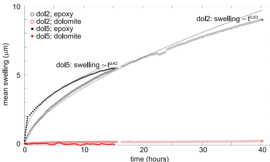
Fig. 5. Average swelling \delta z ( \mu m ) versus time for dol2 and dol5; epoxy in black and dolomite for reference in red. For dol5 there is a 3 bar pressure drop after the first hour (see Table 1), which changed the slope of the swelling curve. The power law fit of the epoxy swelling is shown in black, with the corresponding time exponents. (For interpretation of the references to color in this figure legend, the reader is referred to the web version of this article.)
