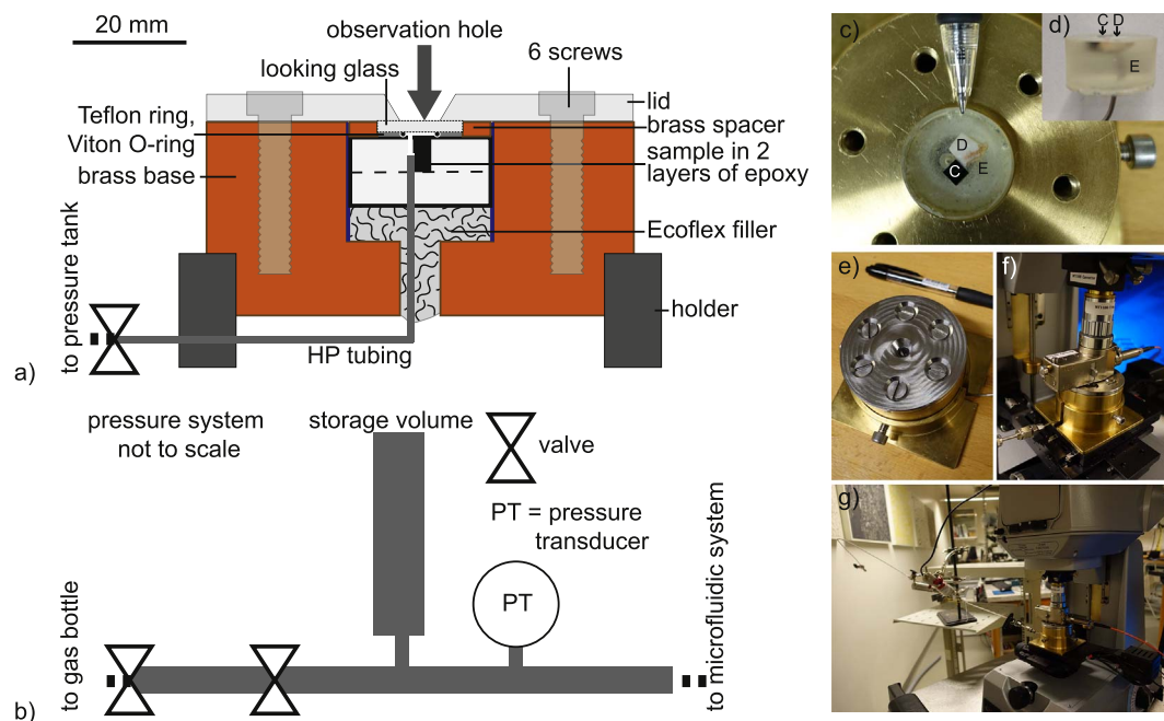
Fig. 1. a) microfluidic sample assembly; b) pressure system, not to scale; c) top view of dolomite (D)/epoxy (E)/coal (C) sample (used for dolcoal1, 2 and 3), pen for scale; d) side view of c); e) assembled pressure device; f) assembly underneath the white light interferometer; g) assembly plus pressure vessel under the white light interferometer.
