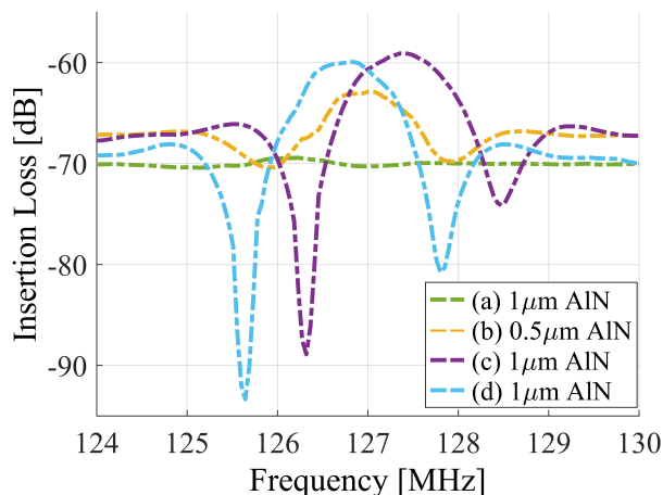
Figure 2.9: AlN thin films of different thickness and sputtered at different temperatures (a) 50 0 C (recipe 1), (b), (c) and (d) 400 0 C (recipe 2). The (c) AlN sample is sputtered continuously whereas the (d) film is sputtered discontinuously and interrupted by the extra cleaning step for the target.
