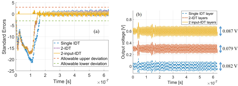
Figure 6.17: (a) The unstable vibration detection of the mechanical waves using the cumulative sum method [28, 29] and (b) output voltages of the novel M-SAW devices and the conventional SAW device (0.3 V offset in Y axis has been added to separate the signals).
