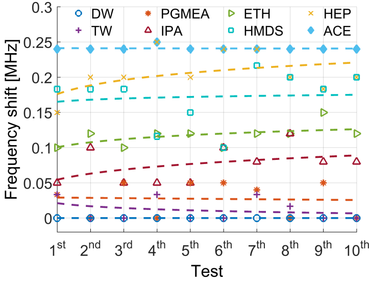
Figure 4.10: Frequency shift of the SAW transducer for different liquids tested.
