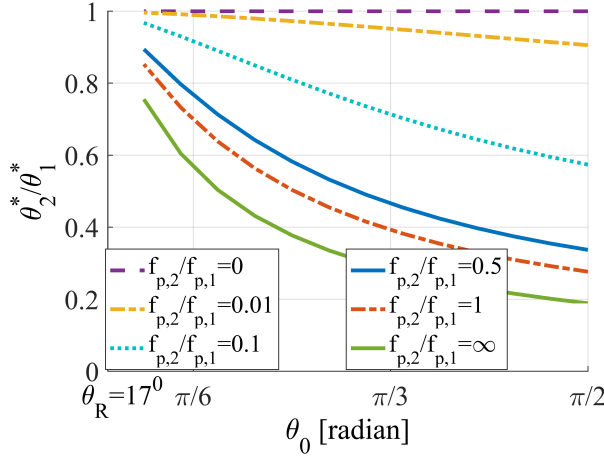
Figure 3.5: The dependence of the critical contact angle ratio \frac{\theta_2^*}{\theta_1^*} on the initial contact angle corresponding to various values of the pinning forces.
