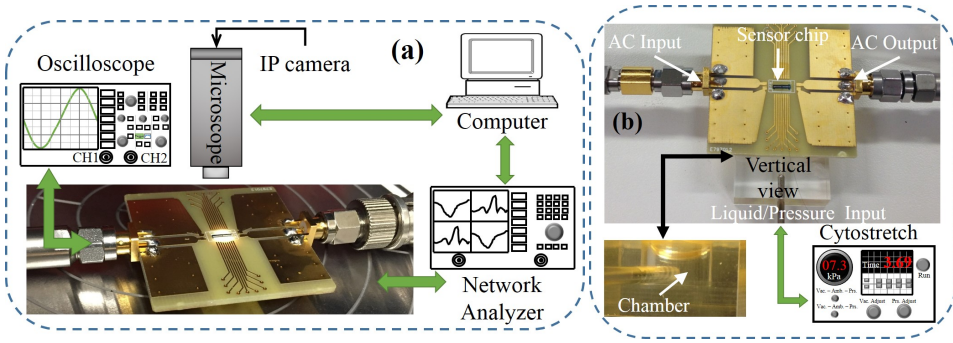
Figure 5.10: Measurement setup for testing (a) evaporation and (b) changeable pressure and density.
