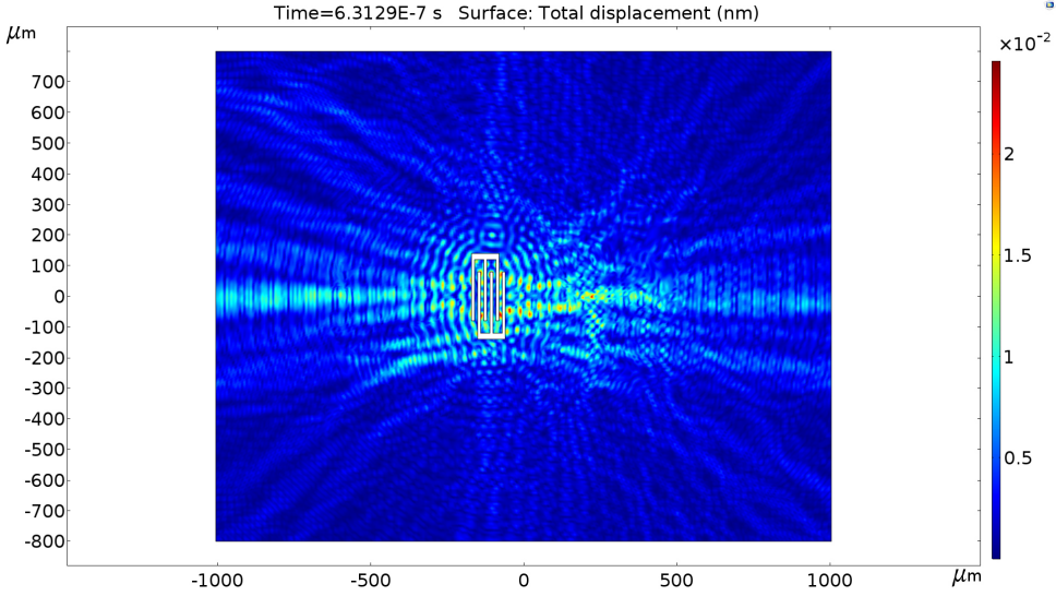
Figure 6.1: Total displacement of the SAW beam generated by three pairs of IDTs.
