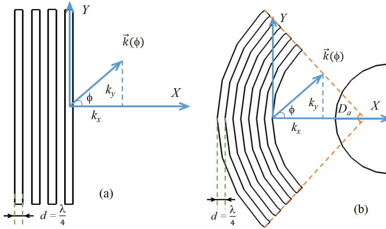
Figure 6.3: (a) Conventional IDTs and (b) FIDTs with circular shape.
