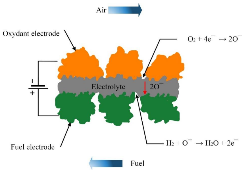
Figure 1.1. SOFC technology
