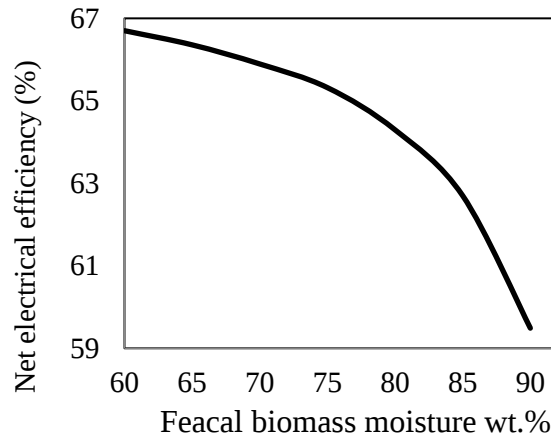
Figure 2.7. Net electrical efficiency as a function of initial biomass MC 60–90 wt.% dried to 30 wt.%.
