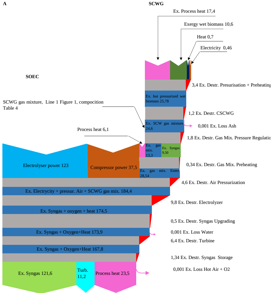
Figure 4.8. Exergy flow diagram (kW) of the SCWG–rSOC system at j = 3.4 A cm -2 , T = 680^{\circ}\text{C} , P = 20 bar, biomass moisture content = 95 wt.%. A) SCWG– rSOC EL mode, B) SCWG– rSOC FC mode with mixed syngas, and C) SCWG–rSOC FC mode with fresh syngas.
