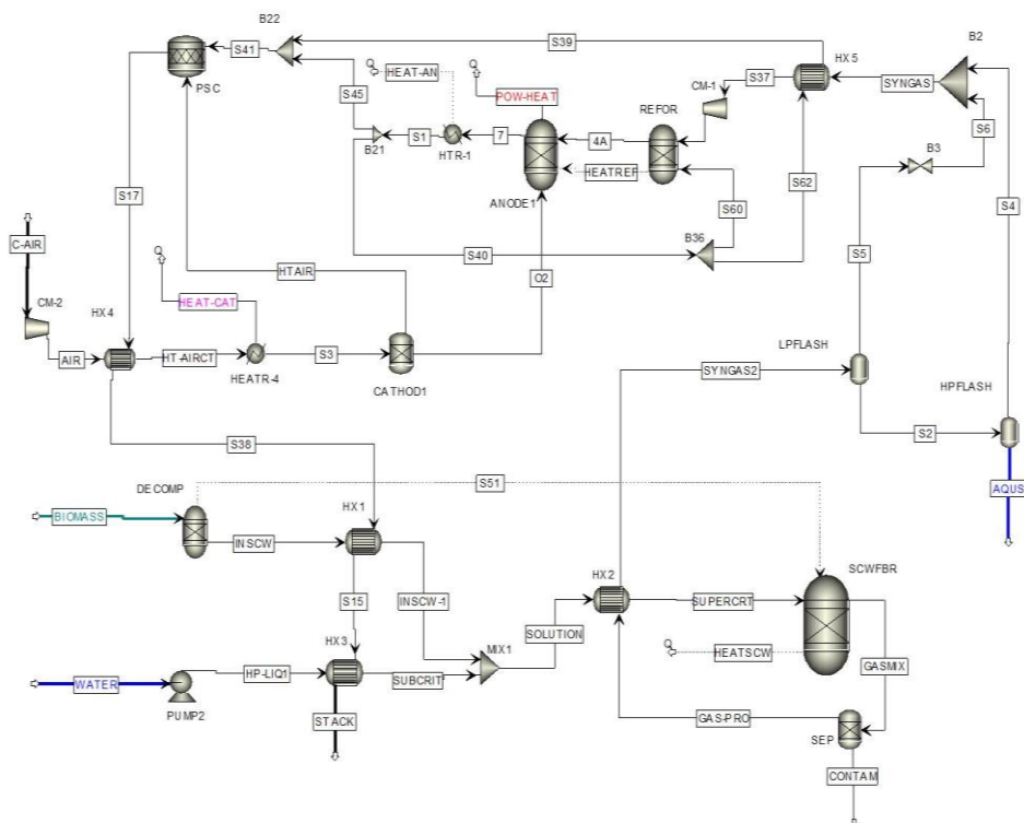
Figure 3.3. Aspen Plus process flow diagram of the supercritical water gasification (SCWG)– solid oxide fuel cell (SOFC) system.
