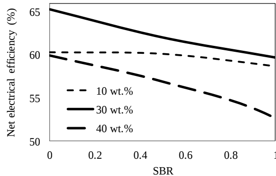
Figure 2.4. Effect of the SBRPG on system net electrical efficiency at 10, 30, and 40 wt.% MC feed to the PG; T = 1100^{\circ}\text{C} .
