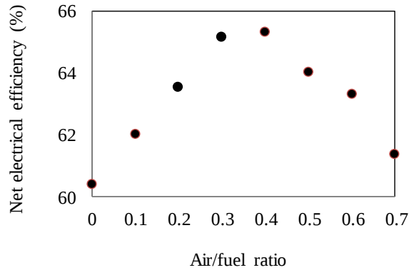
Figure 2.5. Effect of the air/fuel ratio on net electrical efficiency of PG; T = 1100^{\circ}\text{C} and \text{SBRPG} = 0 .
