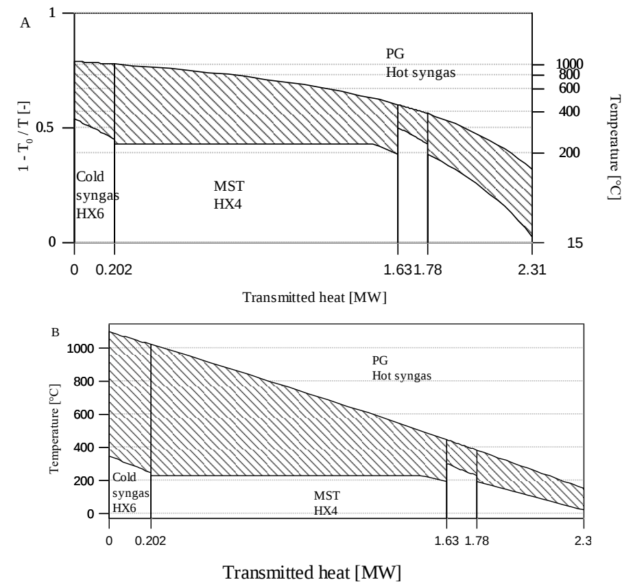
Figure 2.13. QT and value diagrams of the integrated system PG hot syngas.
