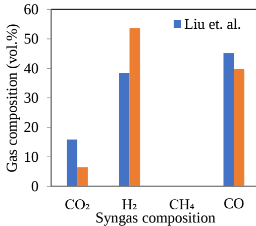
Figure 2.9. Comparison of syngas composition from Liu et al. [69] and the modelled two–stage gasifier, T = 1100^\circ\text{C} , air/fuel = 0.4, MC after dryer = 30 wt.%, and plasma power 0.4 kW.
