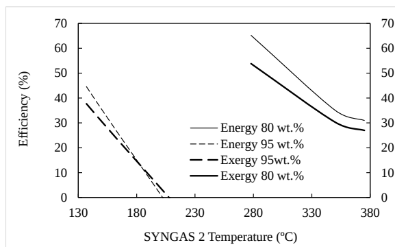
Figure 3.7. Influence of the heat recovery on the supercritical water gasification (SCWG) solid oxide fuel cell (SOFC) efficiency
