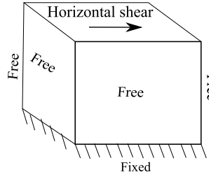
Fig. 6. Synthetic test case: Schematic of the synthetic test case when a horizontal shearing load is applied on the top face. Rest of the faces have stress free boundary conditions. The parameters used in this test case are presented in Table 2.
