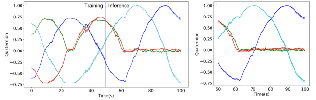
Fig. 7. Quaternion for real data. The solid, dotted and dashed lines correspond to ground truth, integrated and estimated quaternion respectively. The left and right figures are corresponding to scenarios 1 and 2 respectively. In the right figure, the dashed line is obtained by averaging over 50 independent trails.
