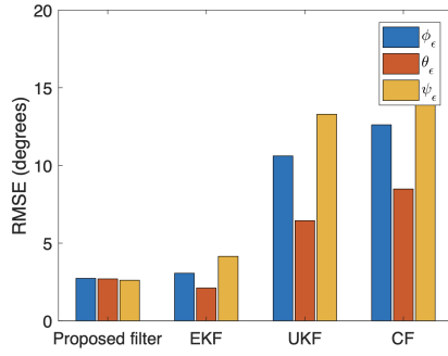
Fig. 4. The RMSE of the proposed filter, Extended Kalman filter (EKF), Unscented Kalman filter (UKF) and Complementary filter (CF) for the inference profiles in Fig. 2(c), 2(c) and 2(d). Because the quaternions double-cover the rotation space which imposes ambiguity in comparison, we use Euler angles instead of quaternions here.
