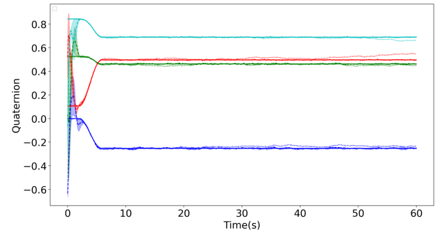
(a) Quaternion for Fig. 2(b)
