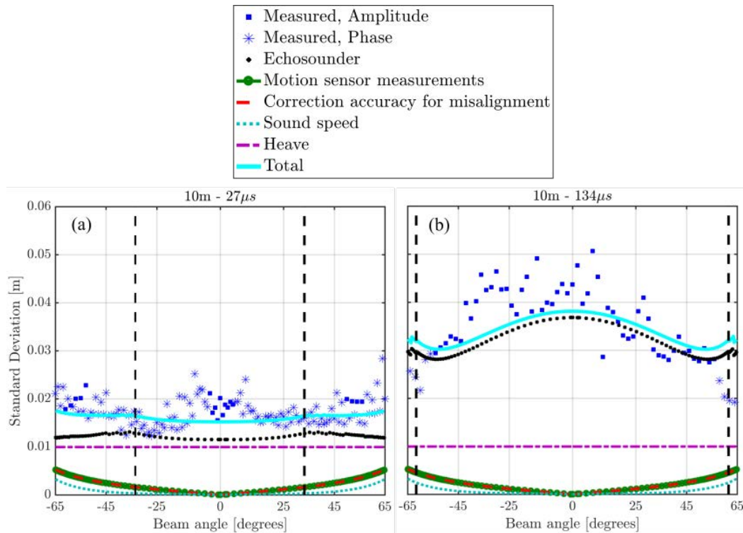
Fig. 3. Measured vertical standard deviation and those predicted for water depth of 10 m and pulse lengths of 27 \mu s (a) and 134 \mu s (b). The black vertical lines shows the location the beam angle where the switch from amplitude to the phase detection occurs according to the criterion of minimum standard deviation.
