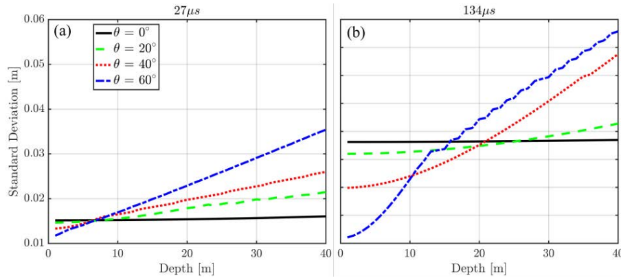
Fig. 1: Predicted depth uncertainty as a function of depth for pulse length of 27\text{ }\mu\text{s} (a) and 134\text{ }\mu\text{s} (b)
