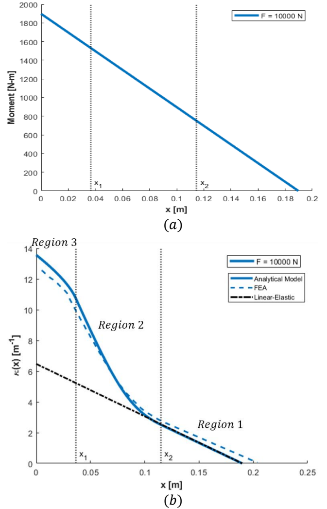
FIGURE 7: MOMENT ALONG DEFORMED CANTILEVER BEAM (A) AND CURVATURE PROFILES COMPARING THE ANALYTICAL BEAM MODEL WITH A LINEAR-ELASTIC BEAM SOLUTION AND FEA (B) FOR A FORCE OF 10000 N
